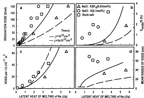
Fig. 2. Measured and calculated dependence of LHM of metallic Na on irradiation dose (a), and the void mean parameters against LHM for different dopants and dislocation densities, \rho . Symbols – experimental data, curves – theory.
