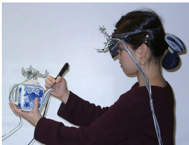
Figure 2. User with AR HMD, modeling teapot with handheld probe. Probe, teapot and HMD are equipped with IR LEDs for opto-electronic tracking.
