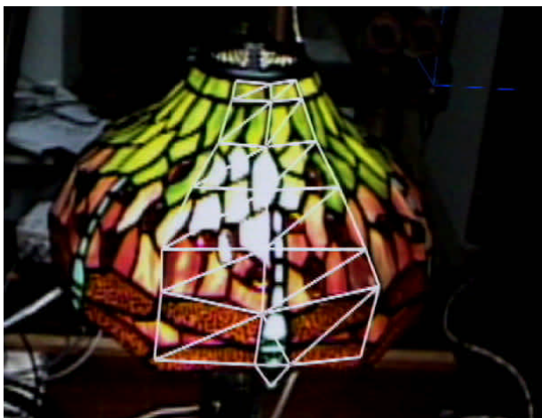
Figure 5. Wire frame model of a 60-degree segment of the lamp overlaid on the video image of the lamp.
