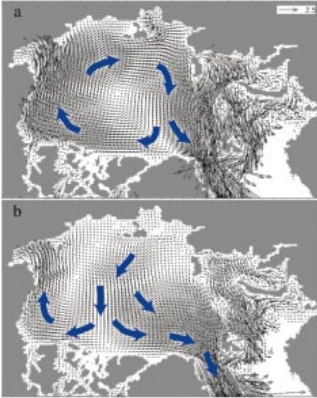
Plate 3. Mean sea ice drift (cm/s) in (a) 1979 at the end of spinup and in (b) 1990-93. Every 3^{\circ} vector in each direction is shown.
