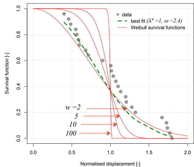
Fig. 5. Survival function for the field pullout tests data. The gray points are the measured data, the green dashed line show the best fit of the Weibull distribution ( \lambda^* = 1 and \omega = 2.4 ), and the red lines show the sensitivity of the Weibull function to the exponent \omega .
