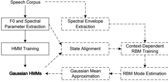
Fig. 1. Flowchart of our proposed method. The modules in solid lines represent the procedures of context-dependent model training in the conventional HMM-based speech synthesis. The modules in dash lines describe the add-on procedures of our proposed method.
