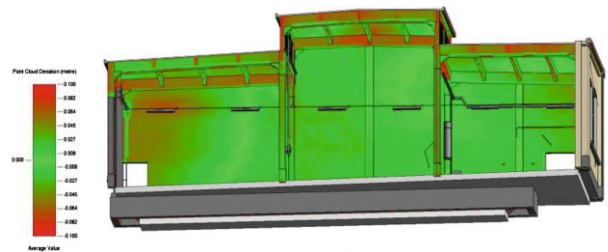
Figure 11. Discrepancy between the point cloud and parametric model. (most of the points that belong to the surface of the walls have a deviation that does not exceed 3 cm).
