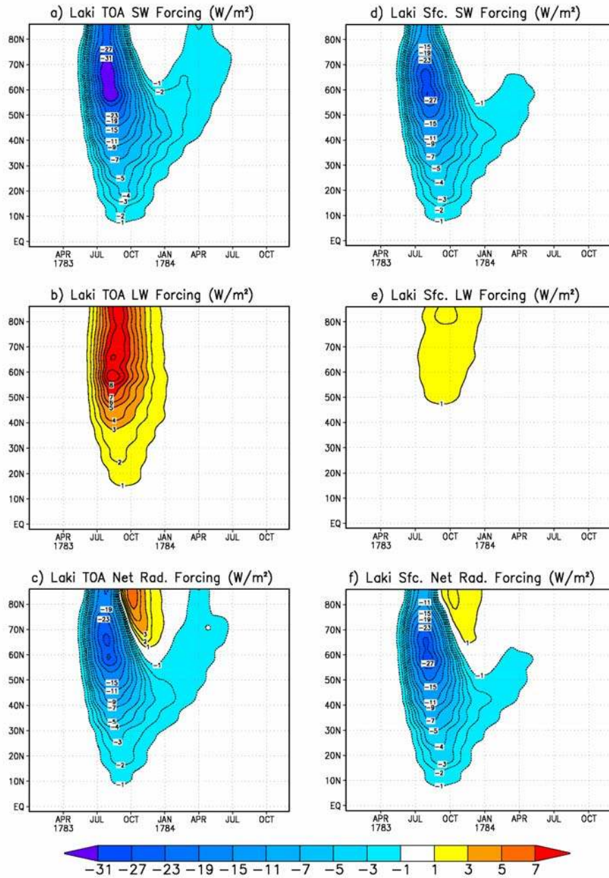
Figure 10. All-sky radiative forcings ( W/m^2 ) calculated for the Laki eruption from January 1783 through December 1784 for the Northern Hemisphere. Shown on the left are TOA shortwave forcing (a) and TOA longwave forcing (b), as well as the TOA net radiative forcing (c). Shown on the right are surface shortwave forcing (d) and surface longwave forcing (e), as well as the surface net radiative forcing (f).
