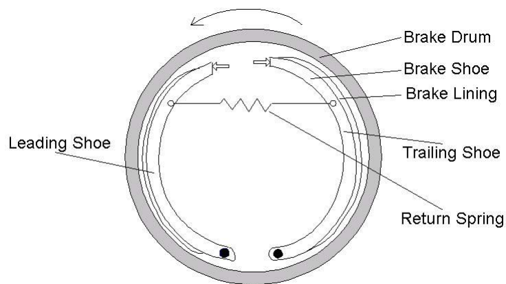
Fig. 3. A schematic of a drum brake
