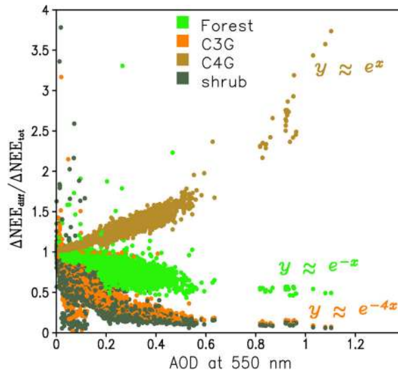
Figure 18. The contribution of the diffuse radiation effect to NEE ( \Delta NEE_{diff}/\Delta NEE_{tot} ) as a function of AOD in the LBAR, but separated with different colors for different types of vegetation. The model data were filtered for cloudiness and precipitation. Additionally, only model points with the same soil water factor within all the three experiments, and soil moisture difference below 0.001 \text{ m}^3\text{m}^{-3} were included. The fitting functions of the \Delta NEE_{diff}/\Delta NEE_{tot} versus AOD for each biome are also shown in the figure.
