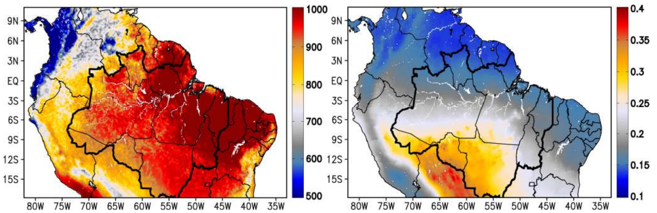
Figure 11. (a) Mean PAR ( \mu\text{mol m}^{-2} \text{s}^{-1} ) at 1600 UTC for September 2010 from DIR+DIF experiment; and (b) the mean diffuse fraction of solar radiation at 1600 UTC for September 2010 as simulated by DIR+DIF. The darker black contour line on the maps delimits the LBAR.
