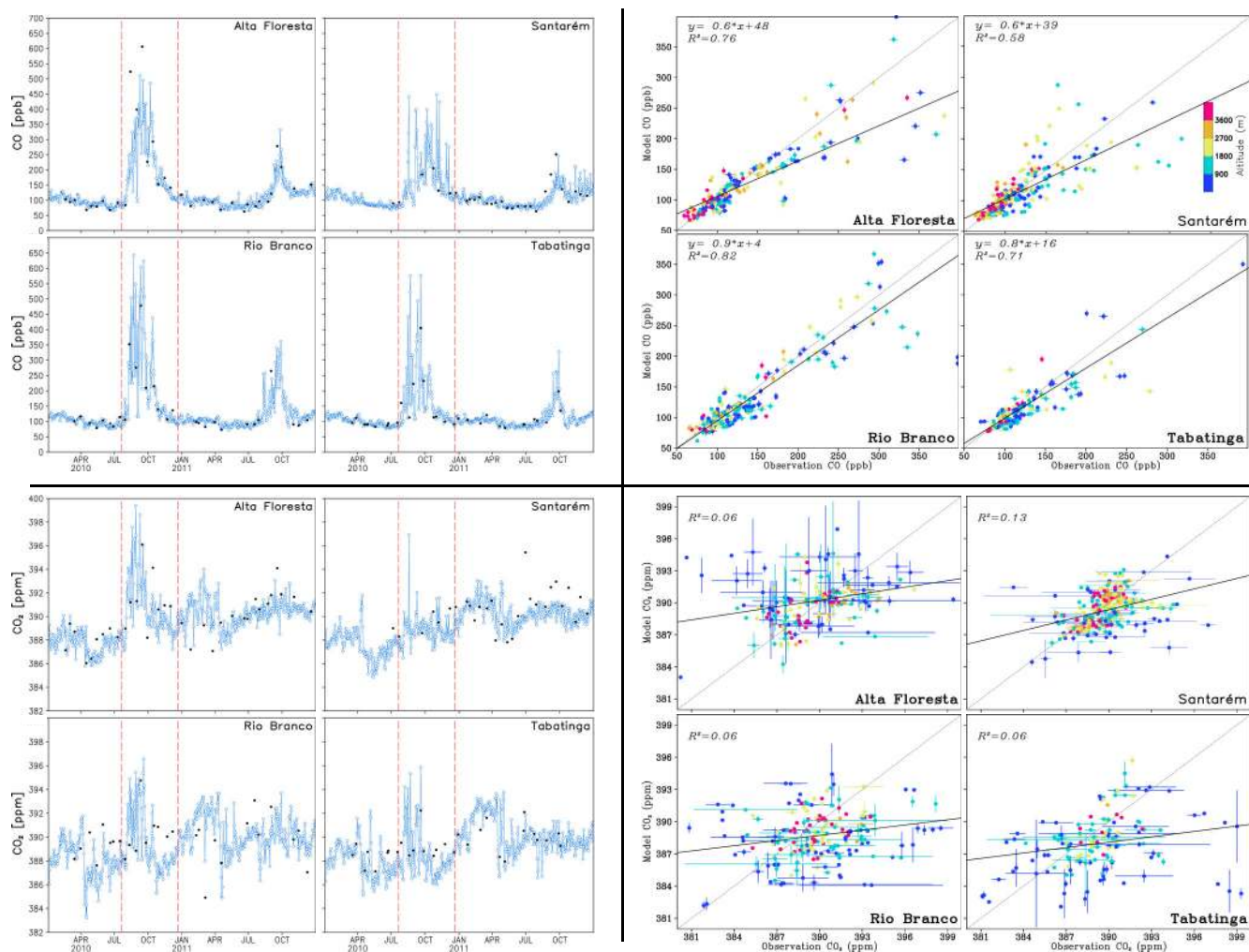
Figure 7. Time series (on the left) and scatter plots (on the right) of CO (ppbv) (on the top) and CO 2 (ppmv) (on the bottom) airborne measured (black dots) and simulated (DIR+DIF experiment, blue dots and line) at Alta Floresta , Santarém , Rio Branco , and Tabatinga (indicated on each plot), at about 2 km above the ground level from April 2010 to October 2011. On the time series, the red dashed lines on the time series indicate the fire season of 2010. On the scatter plots, the colors scale depicts the vertical layers: < 900 m (purple), 900-1800 m (blue), 1800-2700 (green), 2700-3600 (orange), and > 3600 m (pink), and the error bars refer to the standard deviation of the mean values. The locations of the measurement sites are indicated in Figure 2.
