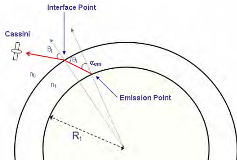
Figure 2. Simple radiometer model showing uniform lossless dielectric layer over an emissive gray body, where n_l is the index of refraction of the surface material, n_0 is the index of refraction of space, \theta_t is the angle of transmission, \theta_i is the angle of incidence, and \alpha_{em} is the anisotropic grazing angle.
