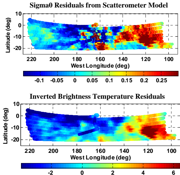
Figure 3. Comparison of the scatterometer model residuals (top) with the inverted radiometer model residuals (bottom) for TA-inbound data reveal the same surface features and demonstrate the anticorrelation of the active and passive radar data. Red means brighter (cooler) than the model, where as blue means darker (warmer) than the model. The optical-bright Xanadu region is on the right and is distinct in both types of data.
