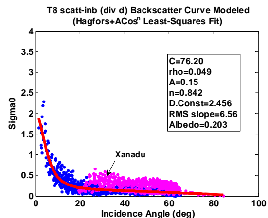
Figure 1. Relative radar cross section is plotted vs. incidence angle. T8-inbound scatterometer data with composite Hagfors-plus-cosine model (red line). Blue data points are from the background surface of the pass. Purple points are return from the radar-bright Xanadu feature and are not considered in the model fitting.
