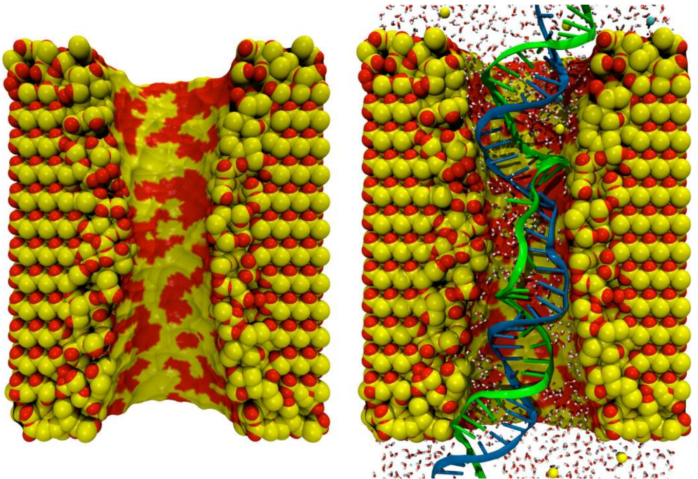
Fig. 4. A silicon dioxide pore (left) created using the Inorganic Builder, and the same pore after including a fragment of DNA and an environment of water and ions (right).
