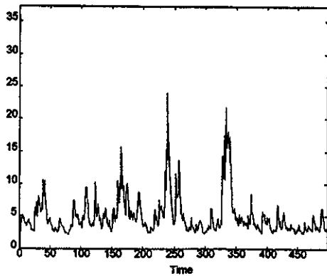
Conditional Covariance
