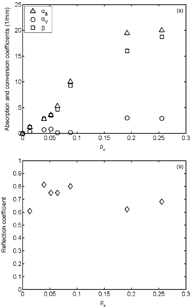
FIG. 3. (a) Dependence of absorption and conversion coefficients on the volume fraction of phosphor in the film and (b) relationship between the reflection coefficient and the volume fraction of phosphor in the film. The absorption coefficient is zero when \rho_v equals to zero because the absorption coefficient of PMMA is effectively zero compared to phosphor particles (Ref. 7).
