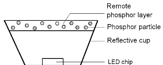
FIG. 1. Remote-phosphor package proposed by Chen (Ref. 4).
