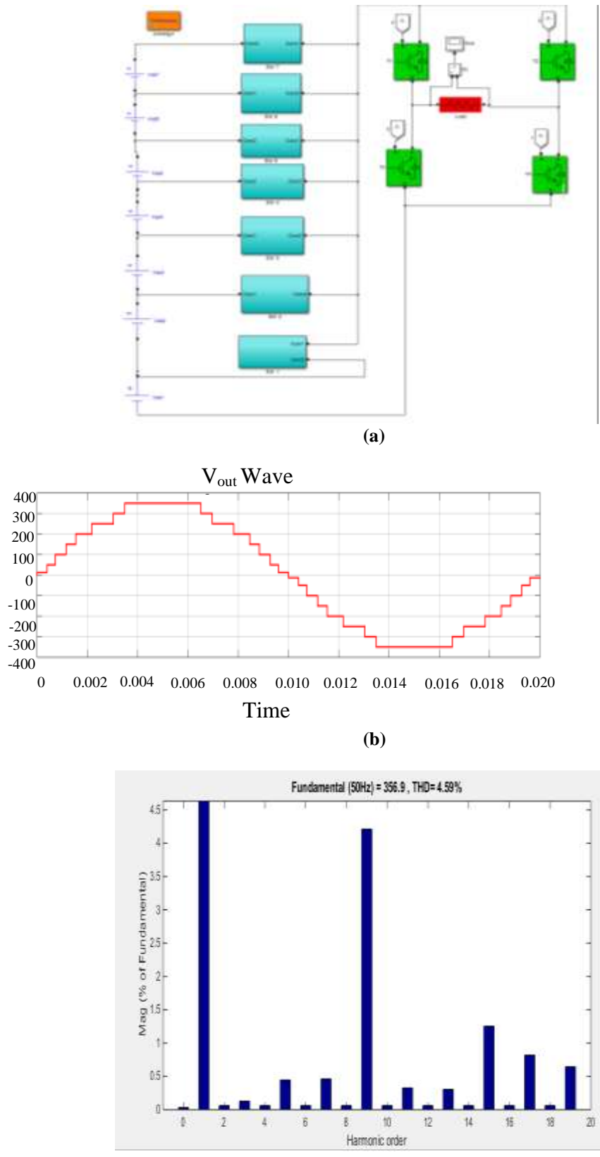
Fig.2.: (a) Simulink Model of Proposed Topology (b) Single Phase Voltage of Proposed Topology (c) Phase Voltage THD in Proposed Topology
