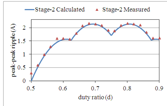
(b) Peak-to-peak ripple in stage-2 channel current
