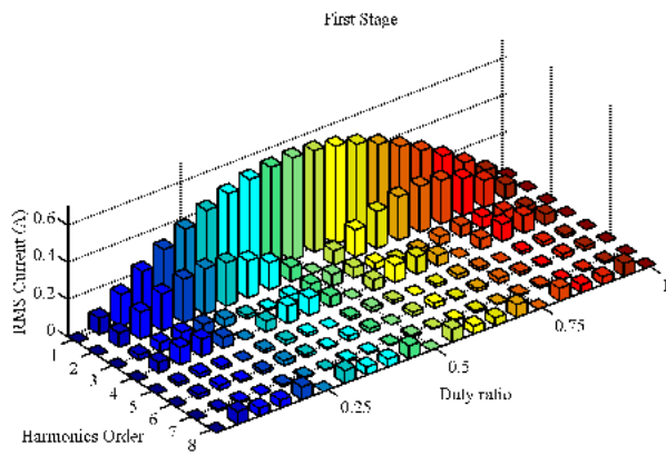
(a) Harmonics components in the stage-1 current
