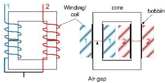
(c) Physical construction of the coupled inductors
