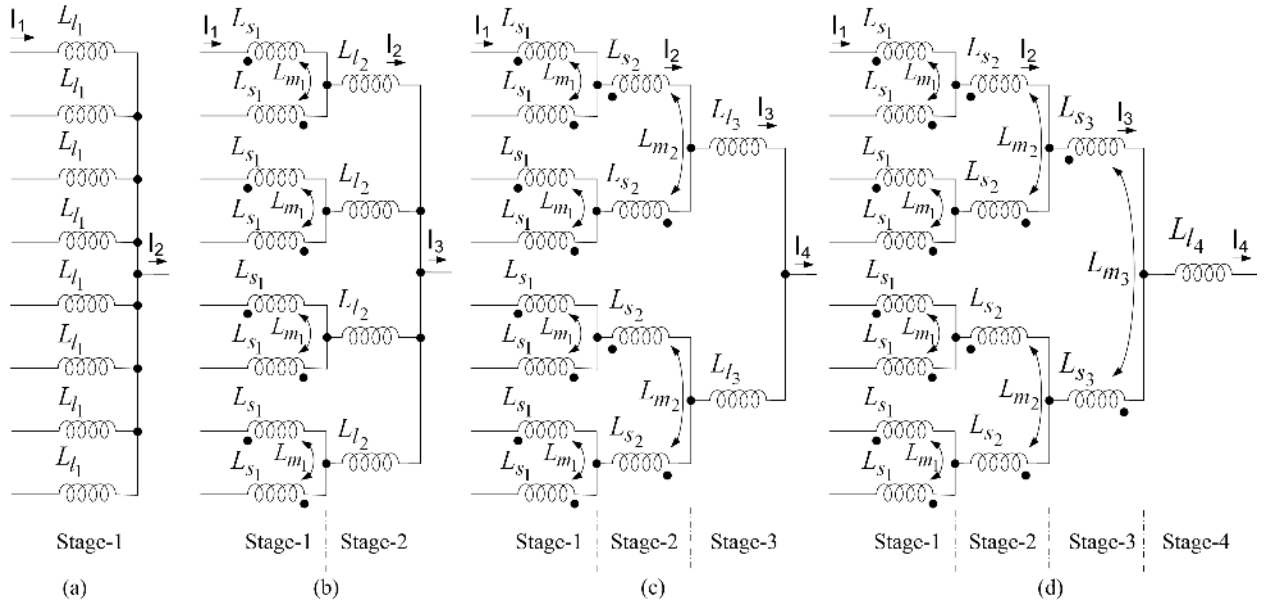
Fig. 2. 4 topologies under comparison: (a) 1-stage topology, (b) 2-stage topology, (c) 3-stage topology, (d) 4-stage topology
