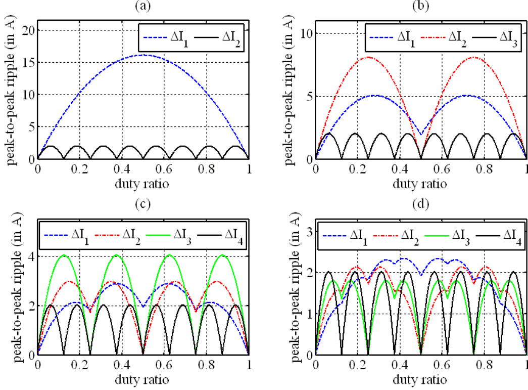
Fig. 3. Peak-to-peak ripple in each channel of various stages in Fig.2: (a) 1-stage topology, (b) 2-stage topology, (c) 3-stage topology, (d) 4-stage topology
