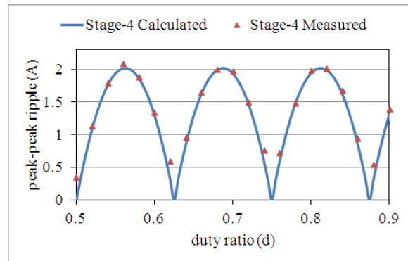
(d) Peak-to-peak ripple in stage-4 channel current
