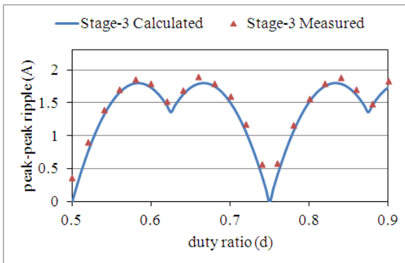
(c) Peak-to-peak ripple in stage-3 channel current
