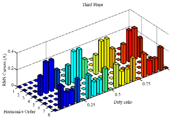
(c) Harmonics components in the stage-3 current
