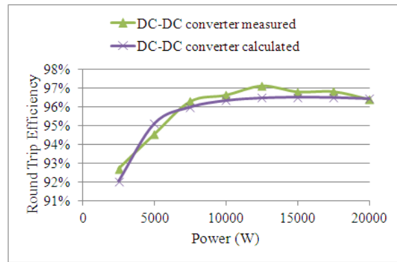
(c) Evaluated and calculated round-trip efficiency of dc-dc converter
