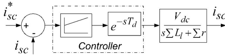
(c) Simplified block diagram of the controller plus plant
