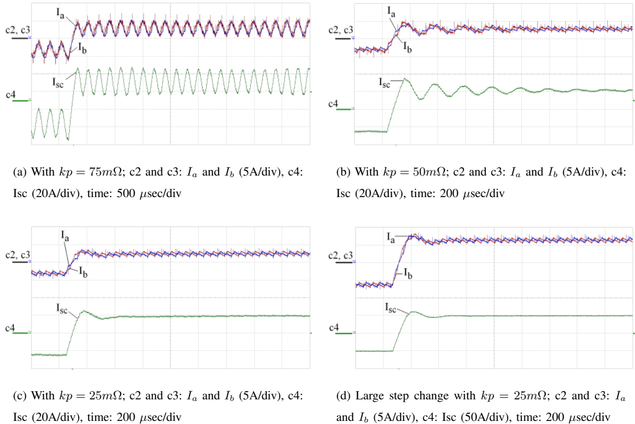
Fig. 12. Measured transient response with various controller gains
