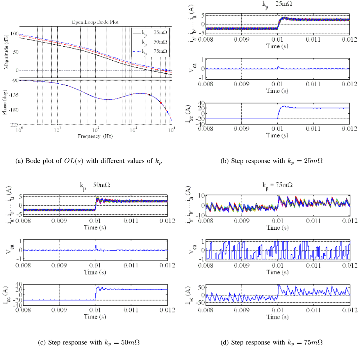
Fig. 5. Bode plot and simulation results
