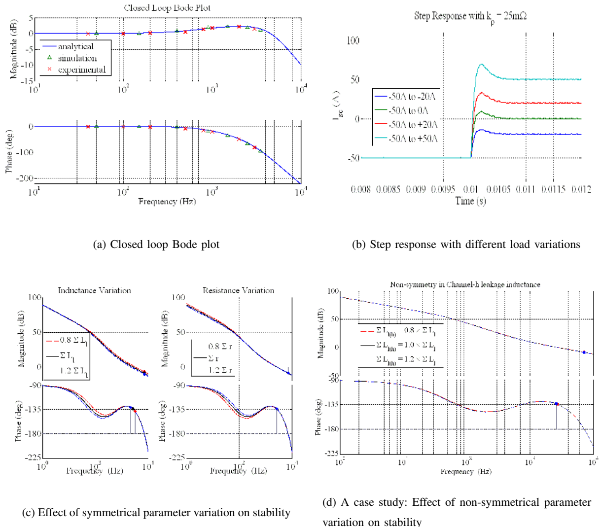
Fig. 6. System performance under different conditions
