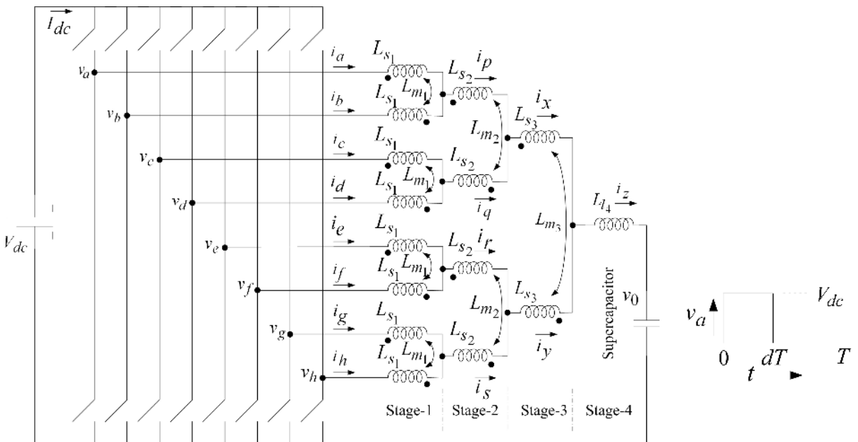
(d) Eight channel interleaved converter with coupled inductors in four stages for supercapacitor interface
