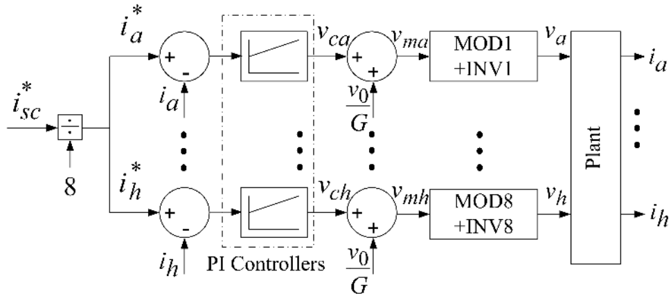
(a) Block diagram of the current controller
