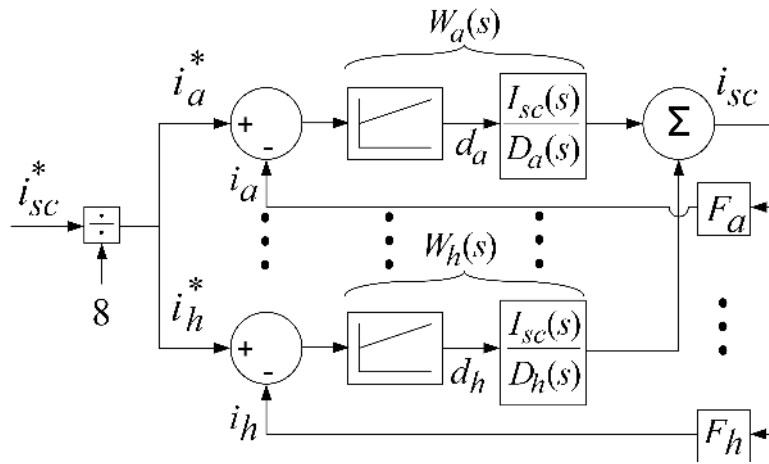
(b) Generalized block diagram of the controller plus plant
