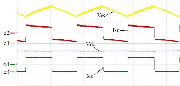
(a) Super capacitor charge discharge cycling at 20kW , c1: V_{sc} (100V/div), c2: I_{sc} (100A/div), c3: V_{dc} (200V/div), c4: I_{dc} (75A/div), time: 20 s/div
