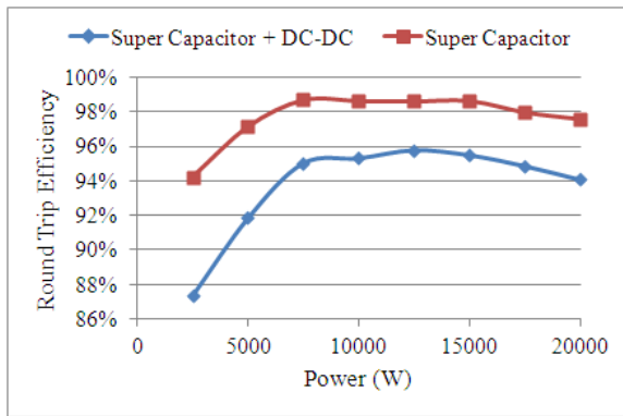
(b) Measured round-trip efficiency of super-capacitor and super-capacitor+dc-dc converter
