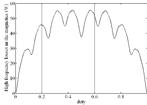
(c) High frequency losses in the magnetic components
