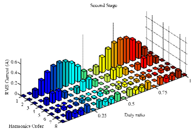
(b) Harmonics components in the stage-2 current
