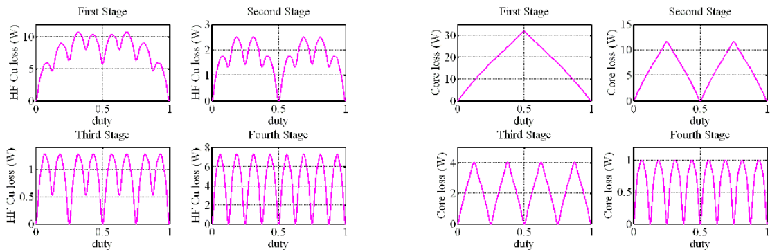
(a) High frequency Copper loss in the magnetic components
