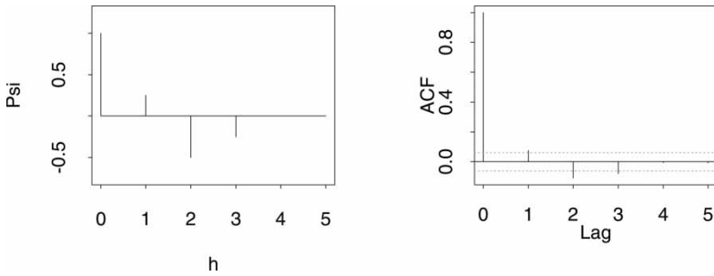
Figure 5. Left-hand plot: \Psi_{-2}(h) for Haar wavelets for h = 0, 1, \dots, 5 . Right-hand plot: sample a.c.f. of F_{i,T} at lags 0, 1, \dots, 5
