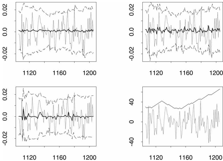
Figure 8. Top left, top right and bottom left: the actual series (dotted line), one-step ahead forecasts (solid line) and 95% prediction intervals (dashed lines) for AR(1) + GARCH(1, 1), AR(16) + GARCH(1, 1) and LSW, respectively. Bottom right: actual series \times 2000 and the evolution of bandwidth h
