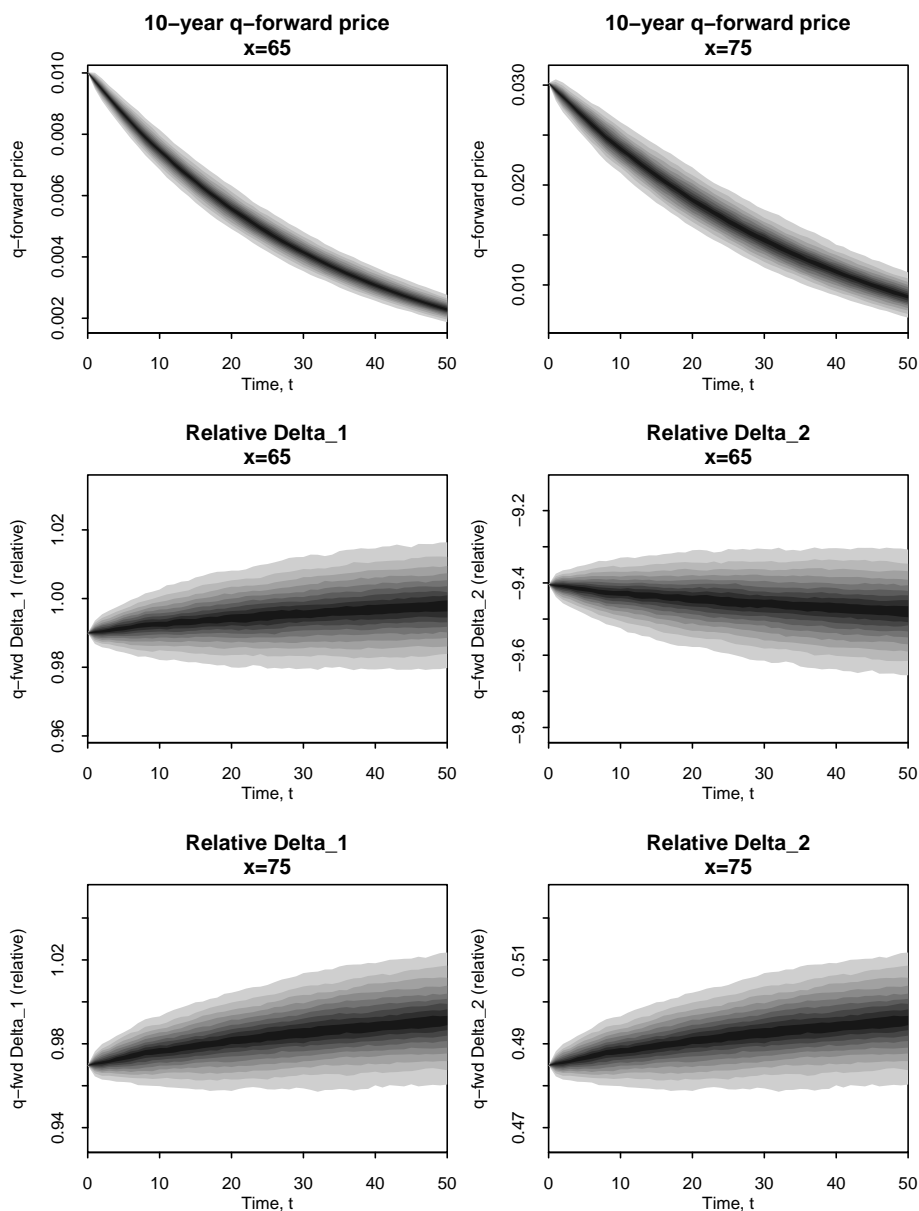
Figure 7: Top row: Fan charts for q^F((t, t + 9, 65)) and q^F(t, t + 9, 75) respectively. Middle row: \Delta_1(t) and \Delta_2(t) for q^F(t, t + 9, 65) relative to the q -forward price, q^F(t, t + 9, 65) . Bottom row: \Delta_1(t) and \Delta_2(t) for q^F(t, t + 9, 75) relative to q^F(t, t + 9, 75) .
