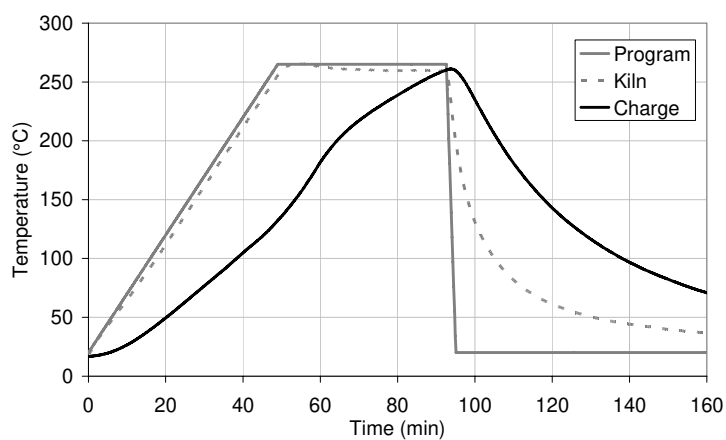
Figure 1: Typical curves of the temperatures recorded during a torrefaction run.
