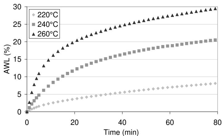
Figure 4: Isothermal thermo-gravimetric analysis of beech wood powder
