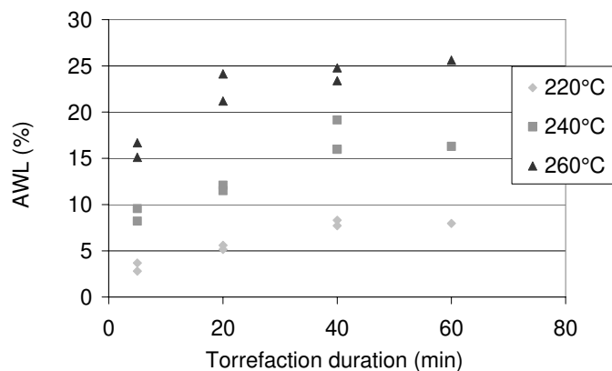
Figure 3: AWL in function of the duration of torrefaction of beech wood chips.
