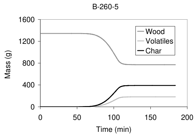
Figure 6: Evolution of wood, char and volatiles according to the simple model.
