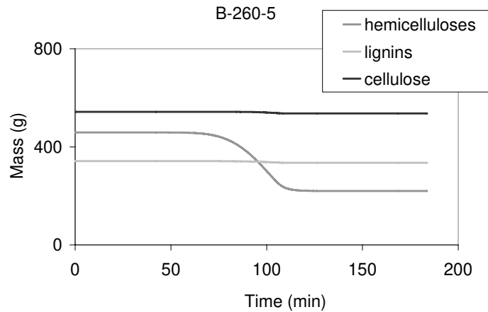
Figure 9: Evolution of hemicelluloses, lignin and cellulose for B-260-5 according to the Rousset model.
