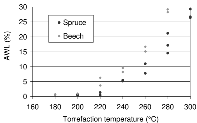
Figure 2: AWL obtained in function of the temperature of torrefaction of beech and spruce wood chips. Samples are kept 5 minutes at torrefaction temperature.
