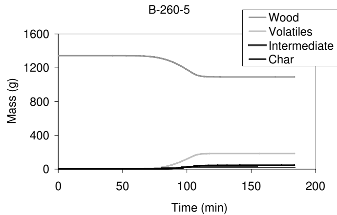
Figure 8: Evolution of wood, volatiles, intermediate compound and char according to the Rousset model.
