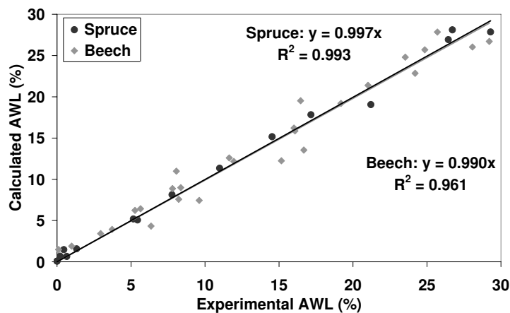
Figure 5: Correlation between experimental AWL and calculated AWL obtained with simple model, for spruce and beech.
