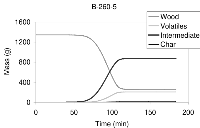
Figure 7: Evolution of wood, volatiles, intermediate compound and char according to the Di blazi-Lanzetta model.
