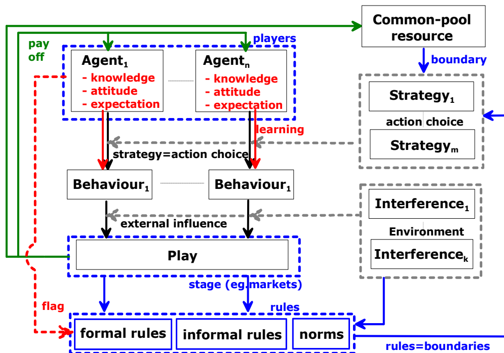
Figure 4. Agent-based conceptualisation.
