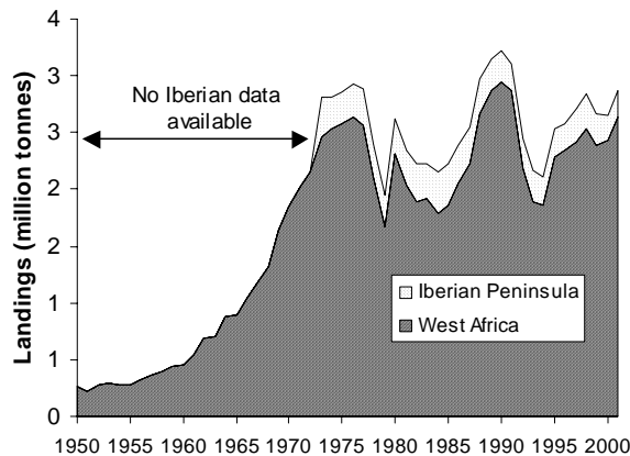
Figure 9-3. Landings of fish (excluding tunas) and shellfish from the Canary Current ecosystem for 1950-2001 and from the Iberian Peninsula for 1973-2001, (Source: FAO and ICES data).
