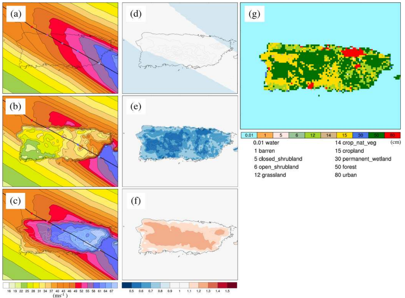
Figure 3. (a–c) Simulated footprints ( \text{m s}^{-1} ) of Hurricane Maria (2017) over Puerto Rico using Willoughby and KW01 with (a) no land (NO_LAND), (b) no terrain height (NO_OROG) and (c) constant surface roughness equal to the ocean value (NO_ROUGHNESS). The hurricane track is shown by the thick black line with input V_{\text{max}} shown every 6 h along the track (coloured dots). Coastlines are shown by the thin black lines and are only included in (a) to aid interpretation. (d) Ratio of Willoughby only to NO_LAND. (e) Ratio of NO_LAND to NO_OROG. (f) Ratio of NO_LAND to NO_ROUGHNESS. (g) Surface roughness (cm) of the land use categories.
