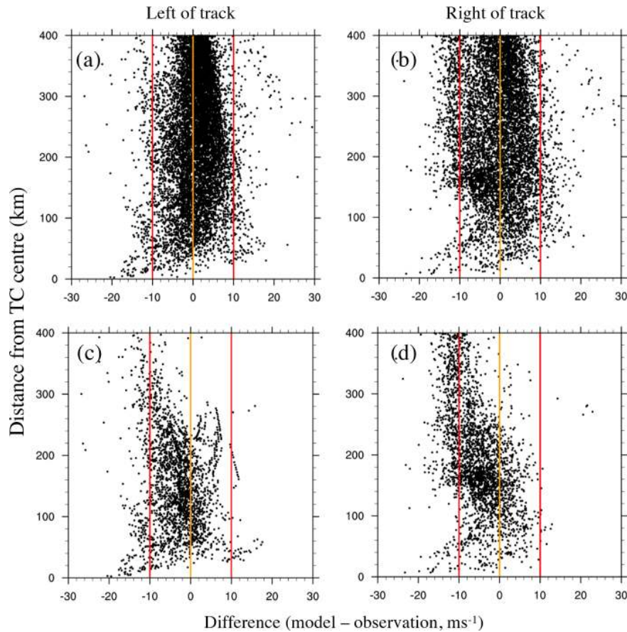
Figure 4. Difference between modelled and observed wind speeds for the eight US storms as a function of distance from the TC centre ( \text{m s}^{-1} ) and split into left of track (a, c) and right of track (b, d). Panels (a) and (b) show all data points, and panels (c) and (d) show only urban data points that experienced observed wind speeds greater than 18 \text{ m s}^{-1} . The orange lines indicate zero difference, and the red lines indicate a positive and negative difference of 10 \text{ m s}^{-1} .
