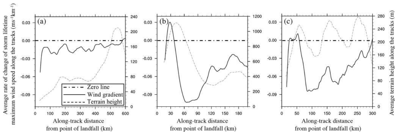
Figure 7. Variation of regional average distance rate of change of wind speed ( \text{m s}^{-1} \text{ km}^{-1} ) and terrain height (m) with along-track distance from the point of landfall (km) for the same regions as shown in Fig. 6; (a) Gulf of Mexico and southeastern US, (b) eastern China and Taiwan, and (c) eastern Australia. All data are smoothed using a 30 point running average. Region-average values are calculated over all tracks within each region. The x axes (along-track distance) are cut off at the point where only three tracks remain. Each panel has the same left- y -axis limits but different right- y -axis limits to better show the ranges of regional terrain height.
