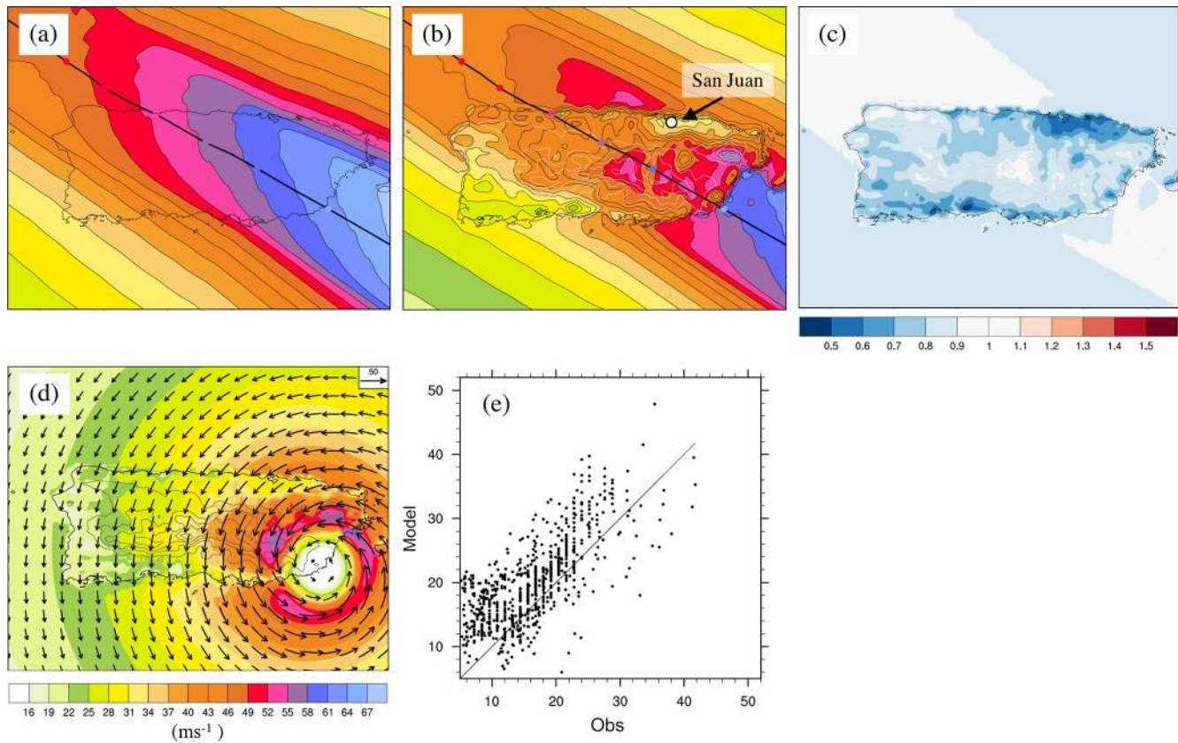
Figure 2. Case study simulation of Hurricane Maria (2017) over Puerto Rico. Simulated footprints ( \text{m s}^{-1} ) are shown using (a) Willoughby only and (b) Willoughby and KW01. The hurricane track is shown by the thick black line with input V_{\text{max}} shown every 6 h along the track (coloured dots). Coastlines are shown by the thin black lines and are only included in panel (a) to aid interpretation. (c) The ratio of Willoughby and KW01 to Willoughby only. (d) A snapshot of the simulation using Willoughby and KW01 at the time of landfall (wind speed is contoured and wind vectors are shown in arrows). Terrain height is contoured every 200 m in panels (b)–(d). (e) A comparison of observed and simulated (Willoughby and KW01) winds.
