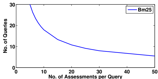
Figure 1: Plot of the Gain Function for BM25.
