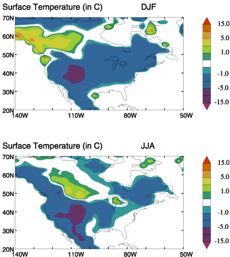
Figure 7. HadAM3 model prediction: difference in surface temperature ( ^{\circ}\text{C} ) over North America between the Pliocene sensitivity experiment and the Pliocene control simulation for both winter (DJF) and summer (JJA) seasons.
