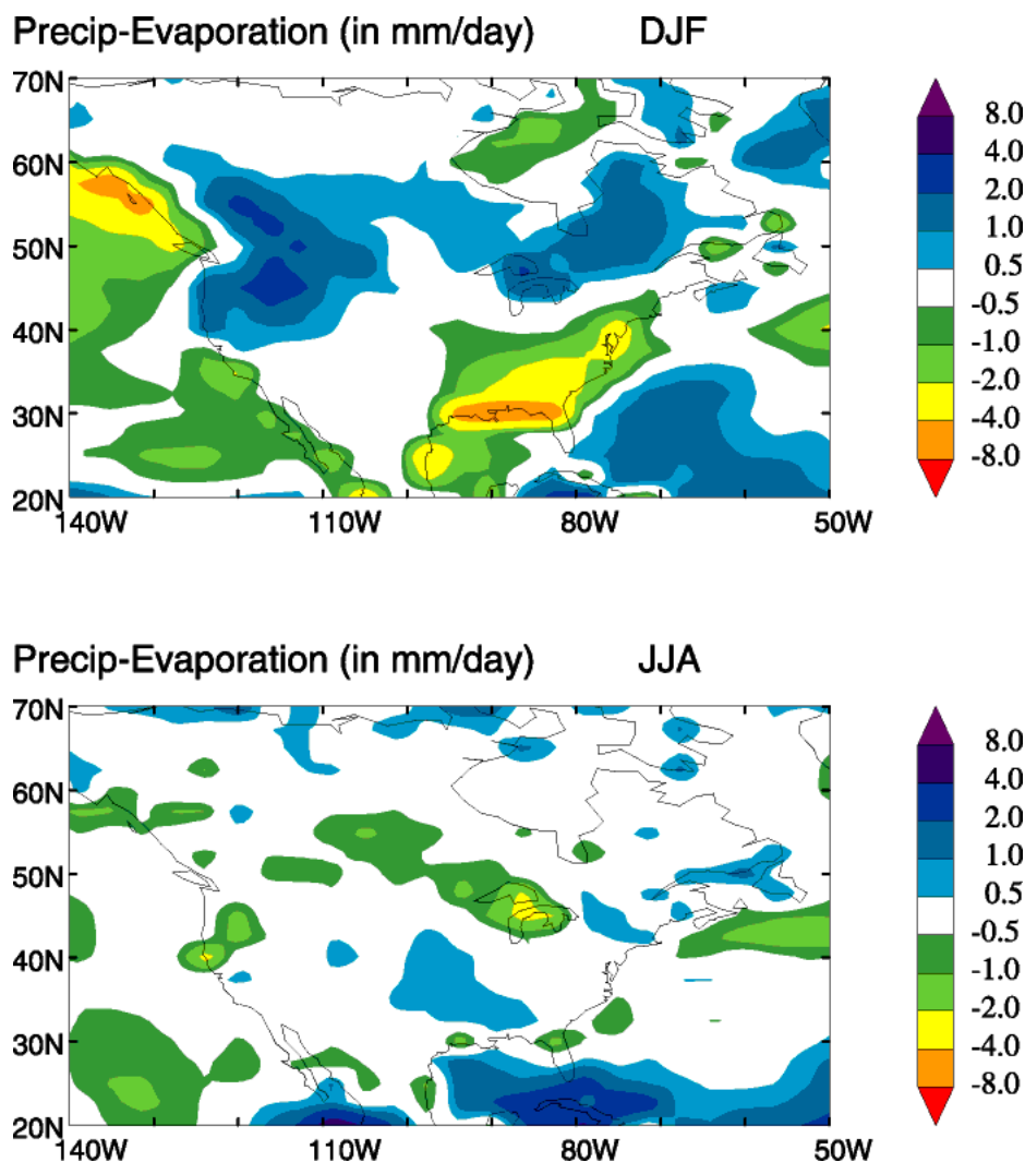
Figure 5. HadAM3 model prediction: difference in P–E values (mm/day) during the middle Pliocene over North America during both winter (DJF) and summer (JJA) seasons.
