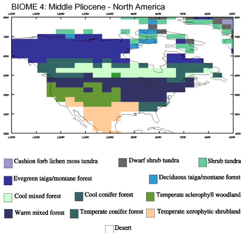
Figure 11. Map of 12 biomes as simulated by BIOME 4 from HadAM3 model's seasonal cycle of temperature, precipitation, and cloud cover over North America for the middle Pliocene.
