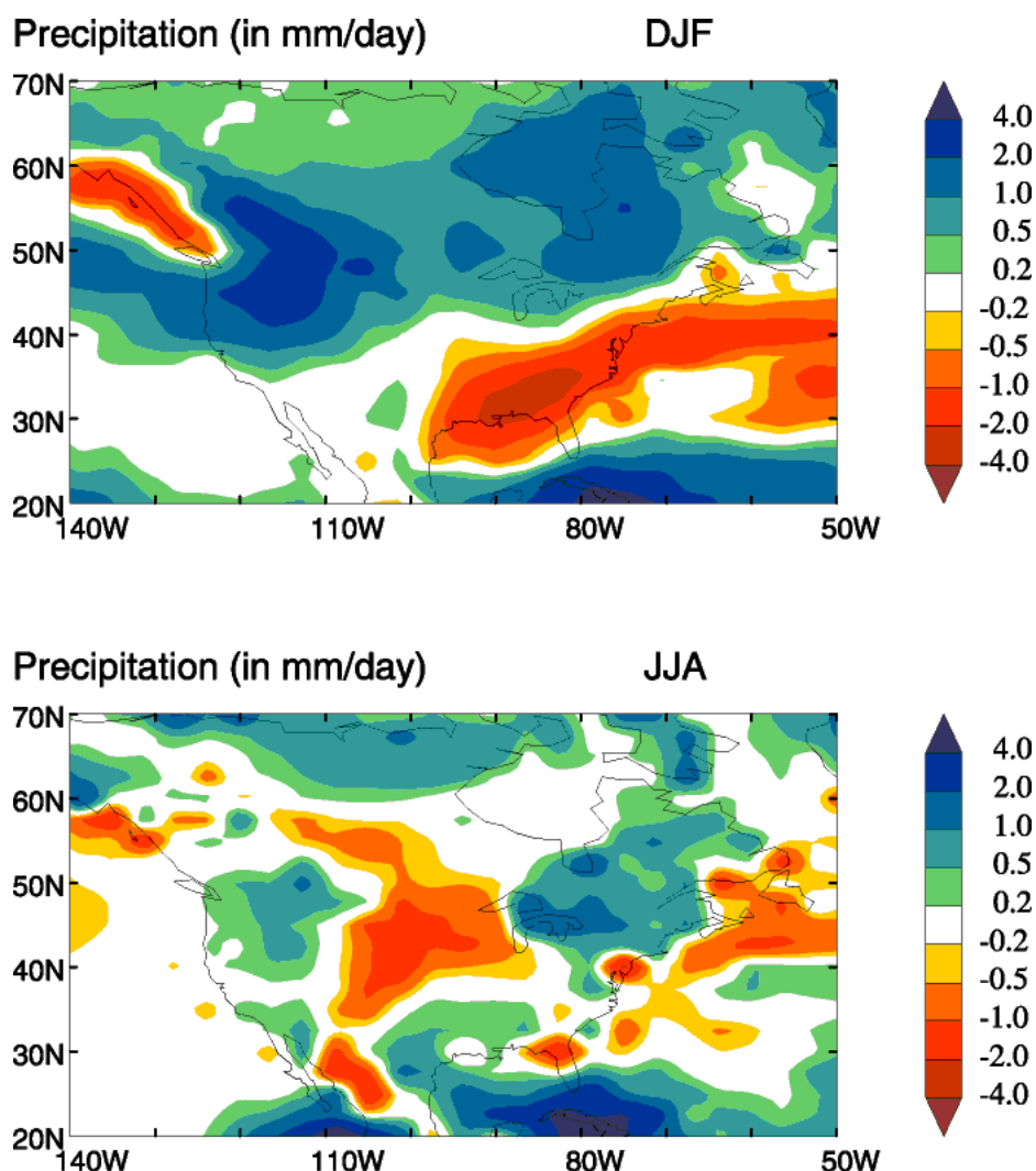
Figure 4. HadAM3 model prediction: difference in the total precipitation rate (mm/day) during the middle Pliocene over North America for both winter (DJF) and summer (JJA) seasons.
