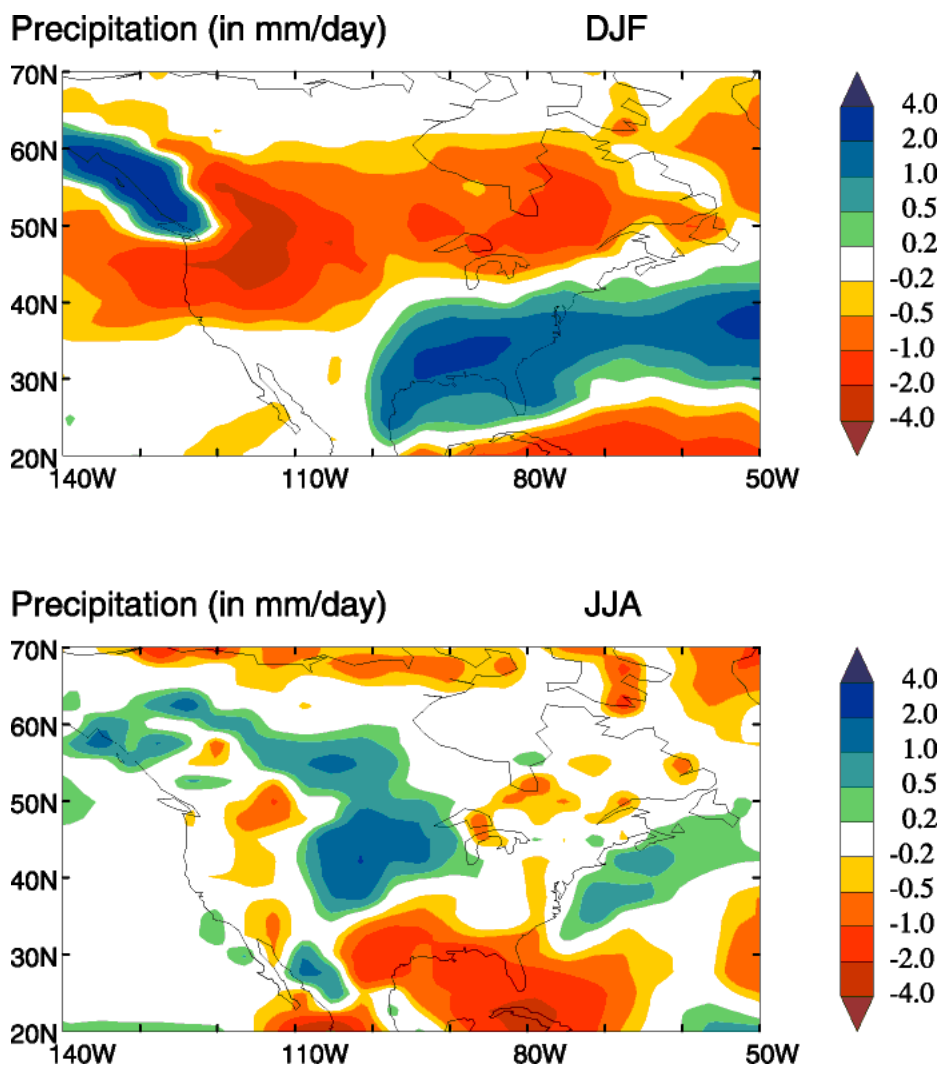
Figure 8. HadAM3 model prediction: difference in the total precipitation rate (mm/day) over North America between the Pliocene sensitivity experiment and the Pliocene control simulation for both winter (DJF) and summer (JJA) seasons.
