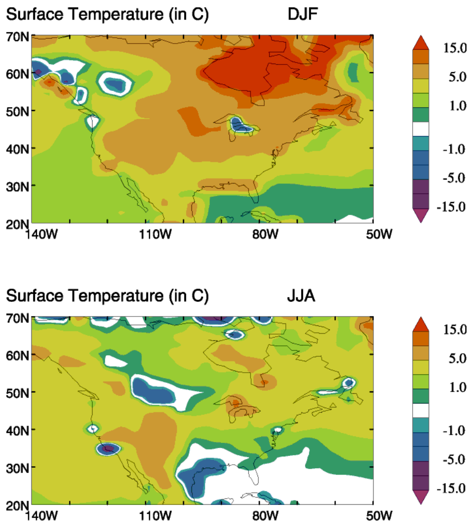
Figure 2. HadAM3 model prediction: difference in surface temperature ( ^{\circ}\text{C} ) during the middle Pliocene over North America for both the winter (DJF) and summer (JJA) seasons.
