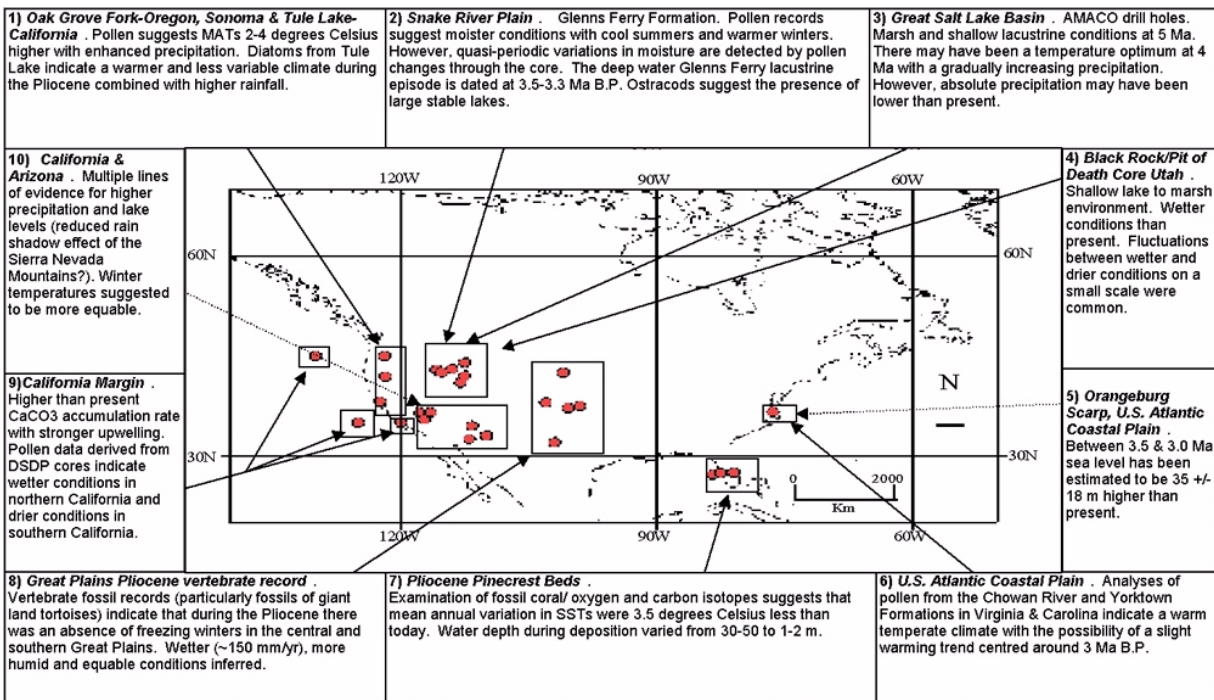
Figure 1. Summary of middle Pliocene palaeoclimatic/palaeoenvironmental evidence derived from the geological record of the United States.
