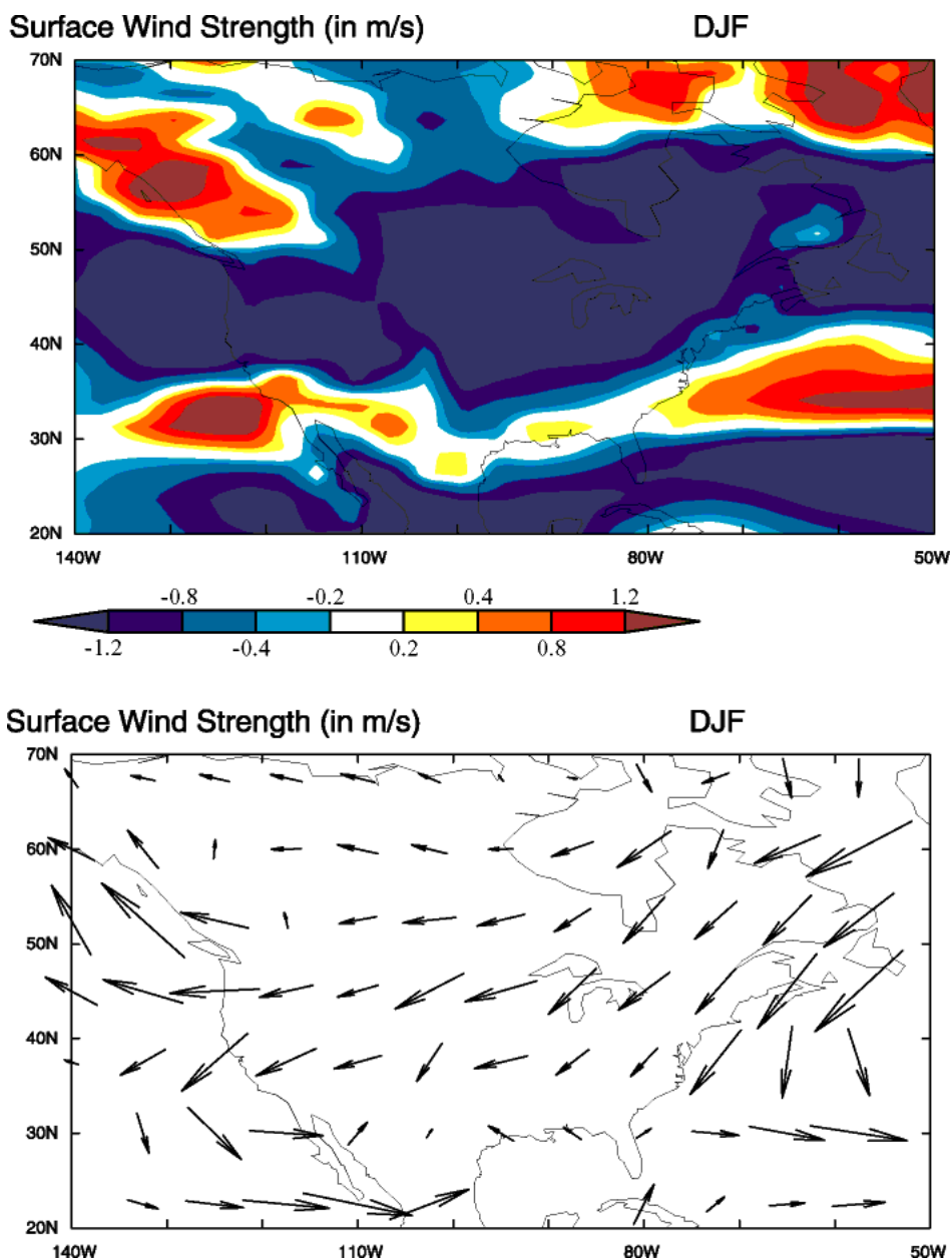
Figure 9. HadAM3 model prediction: difference in surface wind strength ( \text{m/s}^{-1} ) and vector mean winds over North America between the Pliocene sensitivity experiment and the Pliocene control simulation for the winter (DJF) season.
