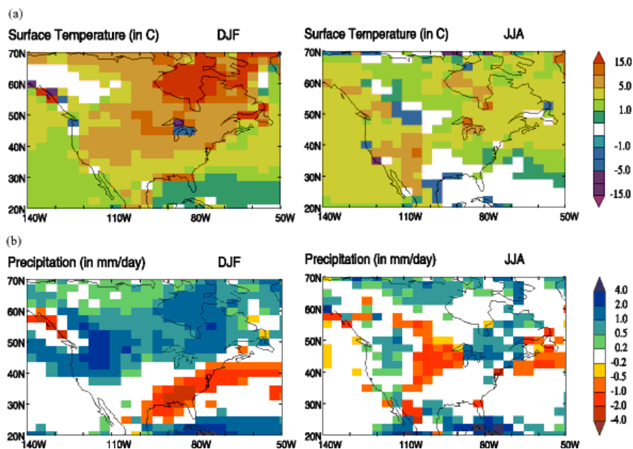
Figure 10. Statistical significance test results for middle Pliocene model simulations of (a) surface temperature ( ^{\circ}\text{C} ) change and (b) total precipitation rate change (mm/day) over North America. Shaded areas show the geographical coverage of statistically significant results (tested to a 95% significance level).
