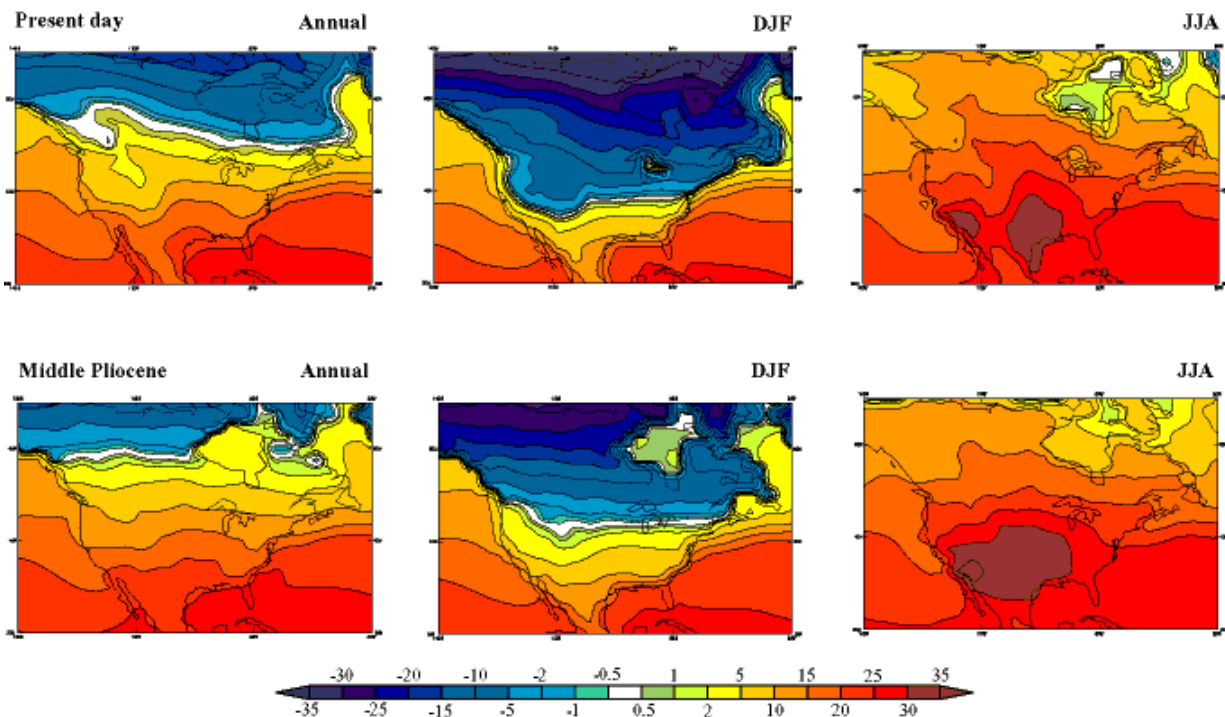
Figure 3. HadAM3 model prediction: present-day and middle Pliocene absolute surface temperatures ( ^{\circ}\text{C} ) over North America for the annual period, winter (DJF), and summer (JJA) seasons.
