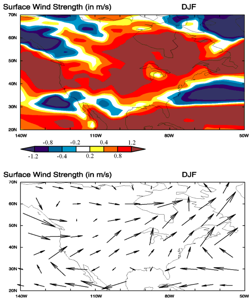
Figure 6. HadAM3 model prediction: difference in surface wind strength ( \text{m/s}^{-1} ) and vector mean winds during the middle Pliocene over North America for the winter (DJF) season.
