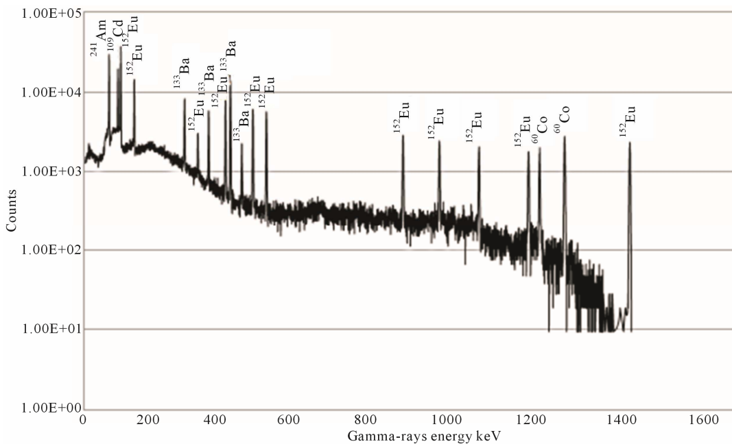
Figure 3. Background spectrum collected from the standard solution.
