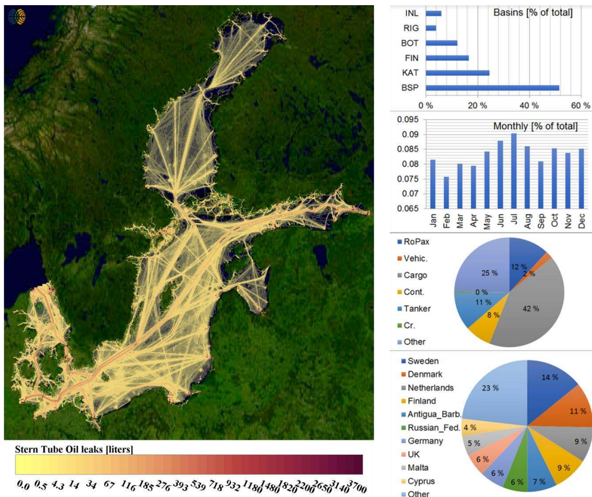
Figure 4: Distribution of the annual stern tube oil releases for year 2012 from the Baltic Sea shipping. Discharge volumes are indicated in liters per map grid area of 5 km 2 . Top right: Share of stern tube oil released in various sub-basins of the Baltic Sea (INL=Inland areas, RIG=Gulf of Riga, BOT=Bothnian Bay and Bothnian Sea, FIN=Gulf of Finland, KAT=Kattegat, BSP=Baltic Sea Proper). Lower bar chart depicts the monthly variation of stern tube oil discharges. Upper pie chart summarizes the contribution of various ship types to stern tube oil releases and the lower pie chart the flag state shares of stern tube oil releases. Map background Landsat-8 image courtesy of the U.S. Geological Survey.
