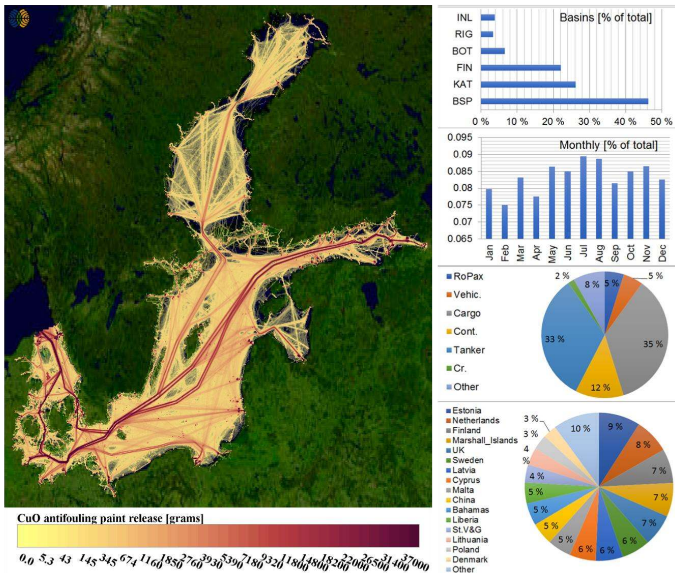
655 Figure 9: Geographical distribution of the emissions of Cu(I)O from ship hull antifouling paints. The values reported by the color scale indicate CuO releases in unit of grams per map grid cell of 5 km 2 . Top right bar chart indicates the share of Cu(I)O releases by sea area (INL=Inland areas, RIG=Gulf of Riga, BOT=Bothnian Sea and Bothnian Bay, FIN=Gulf of Finland, KAT=Kattegat, BSP=Baltic Proper). Lower bar chart describes the monthly variation of CuO releases. Upper pie chart illustrates the estimated share various ship types and the lower pie chart the flag state contributions to CuO releases. Map background Landsat-8 image courtesy of the U.S. Geological Survey.
