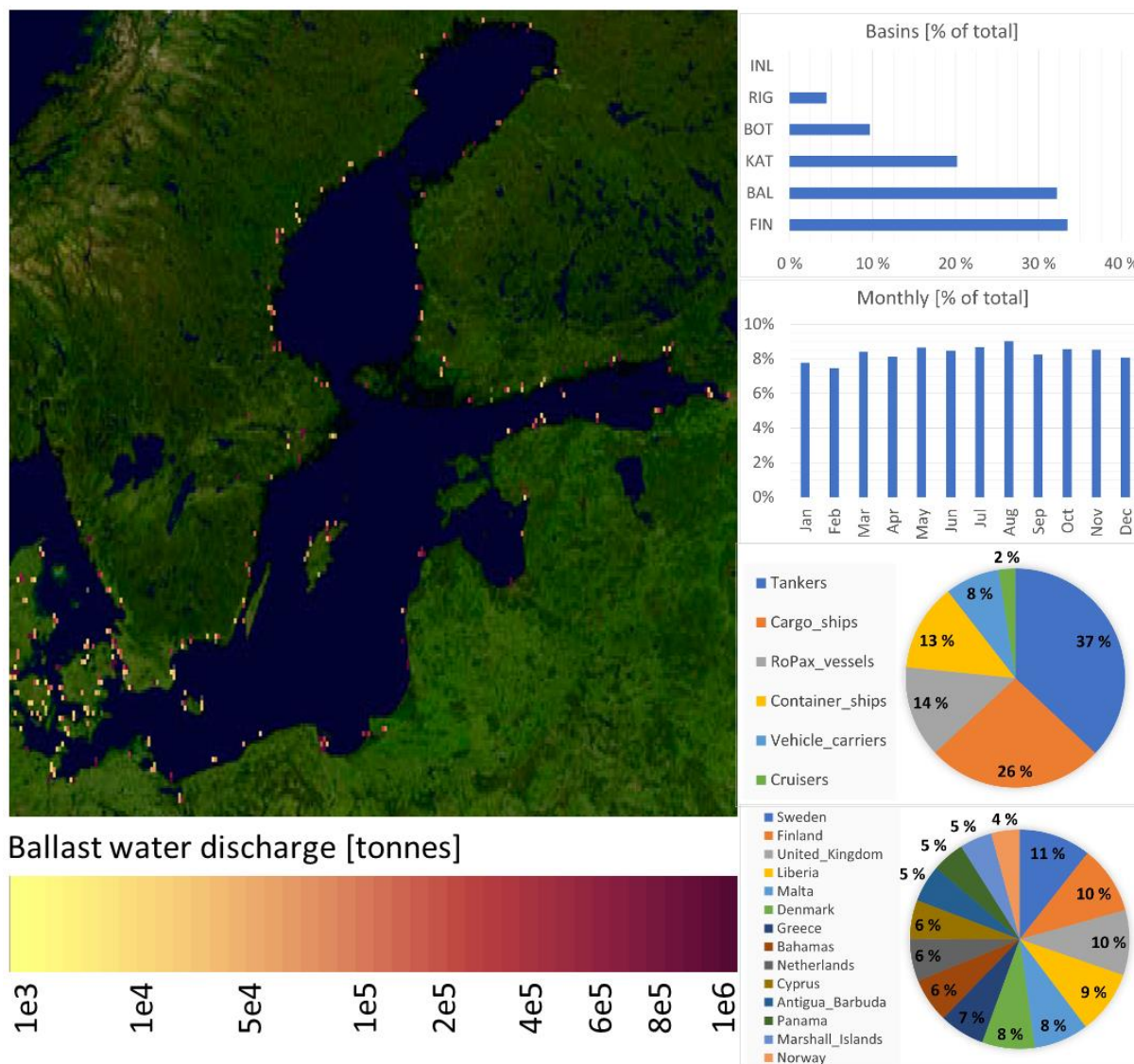
600 Figure 8: Distribution of the annual ballast water releases for year 2012 from the Baltic Sea shipping. Discharge volumes are indicated in tonnes per map grid area of 40 km 2 . Note the change of map resolution to highlight ballast water discharge locations on this map. Top right: Share of ballast water released in various sub-basins of the Baltic Sea (INL=Inland areas, RIG=Gulf of Riga, BOT=Bothnian Bay and Bothnian Sea, FIN=Gulf of Finland, KAT=Kattegat, BSP=Baltic Sea Proper). Lower bar chart depicts the monthly variation of ballast water discharges. Upper pie chart summarizes the contribution of various ship types to ballast water releases and the lower pie chart the flag state shares of ballast water releases. Map background Landsat-8 image courtesy of the U.S. Geological Survey.
