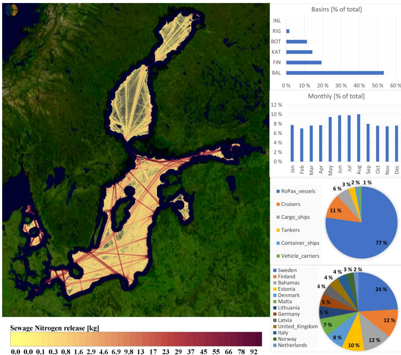
705 Figure 11: Sewage nitrogen discharges from ships during 2012 in unit of kilograms per map grid cell area of 5 km 2 . According to IMO rules, no discharge is allowed closer than 12 nm distance from the coastline. Upper bar chart describes the contributions by sub-basin, lower bar chart the monthly variation. Upper pie chart depicts the ship type and lower pie chart the flag state contributions to sewage nitrogen releases. Map background Landsat-8 image courtesy of the U.S. Geological Survey.
