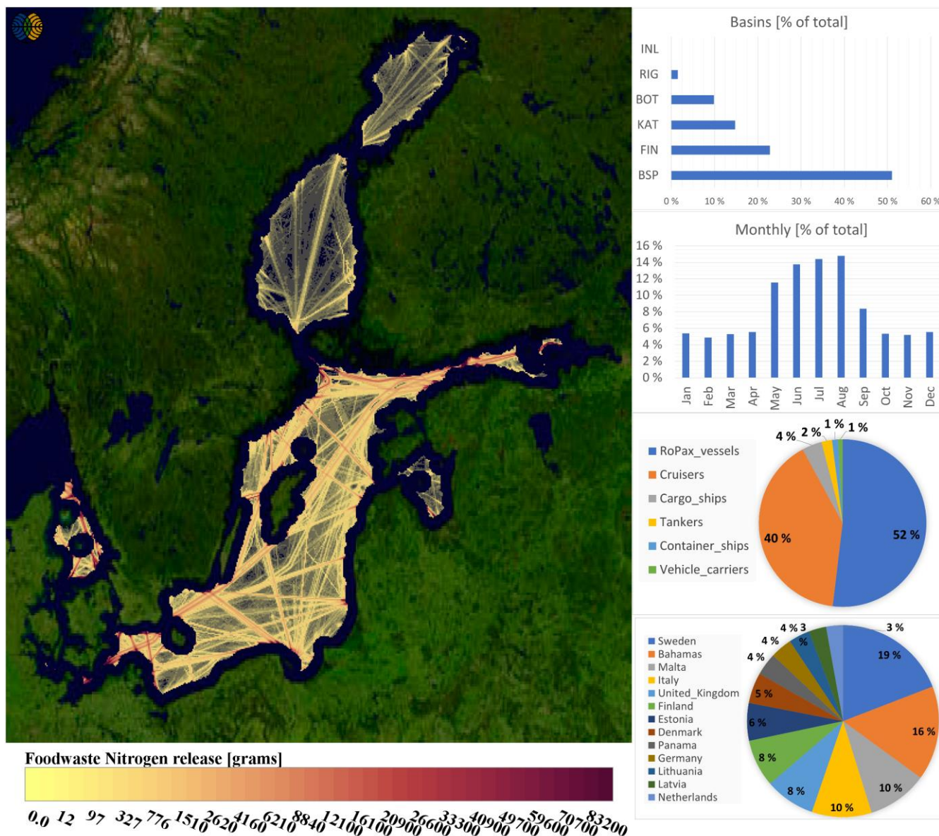
690 Figure 10: Food waste nitrogen discharges from ships during 2012 in unit of grams per map grid cell area of 5 km 2 . According to IMO rules, no discharge is allowed closer than 12 nm distance from the coastline. Upper bar chart describes the contributions by sub-basin, lower bar chart the monthly variation. Upper pie chart depicts the ship type and lower pie chart the flag state contributions to foodwaste nitrogen releases. Map background Landsat-8 image courtesy of the U.S. Geological Survey.
