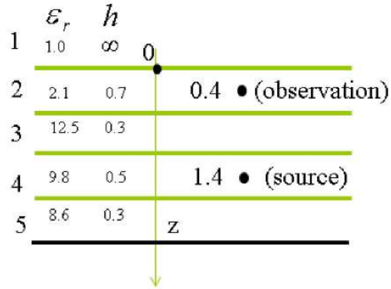
Fig. 12 A five-layer media with source and observation points in the different layer
