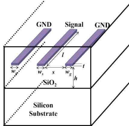
Fig. 1 Coplanar waveguide on silicon interposer
