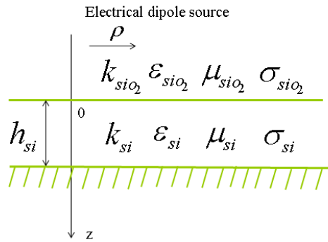
Fig. 4 Geometry and coordinates of layered Si-SiO 2 Media
