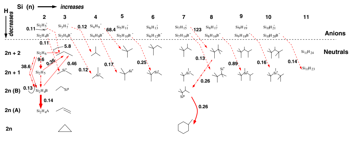
Figure 7. Dominant neutral reaction pathways at steady-state ( T_{gas} = 500 K, N_i = 3 \times 10^9 cm ^{-3} ); the numbers indicate net reaction rates in units of 10^{-15} mol cm ^{-3} s ^{-1} .
