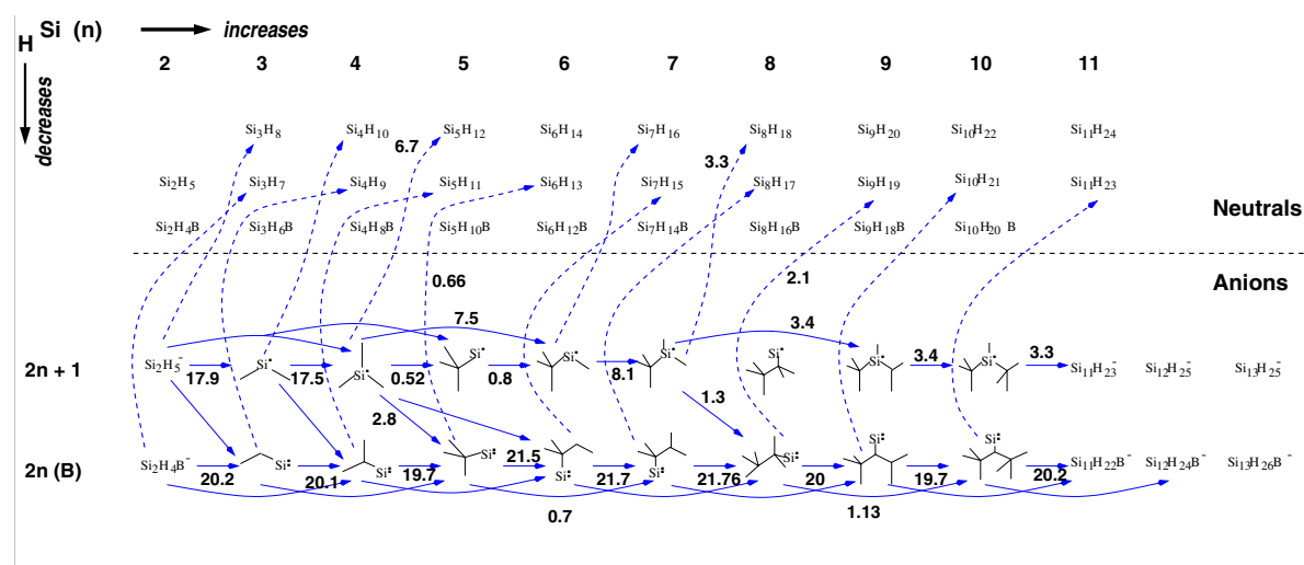
Figure 8. Dominant anionic reaction pathways at steady-state ( T_{gas} = 500 K, N_i = 1 \times 10^{11} cm ^{-3} ); the numbers indicate net reaction rates in units of 10^{-11} mol cm ^{-3} s ^{-1} (all unlabelled reaction rates are of the order 10^{-12} mol cm ^{-3} s ^{-1} ).
