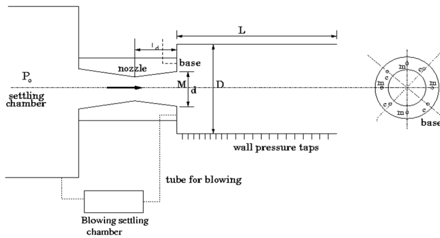
Figure 3. Experimental set up.
