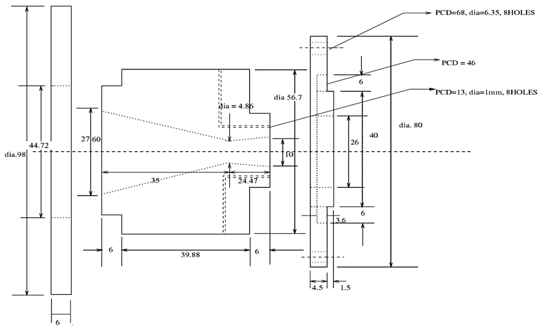
Figure 2. Nozzle design for Mach 3.0.
