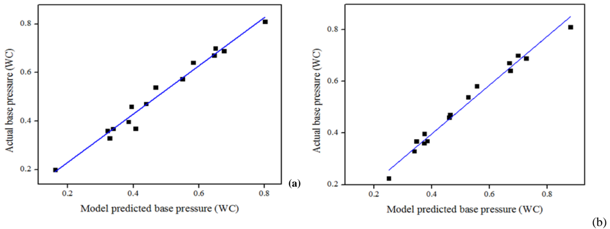
Figure 11. Comparison of model predicted base pressure (WC) with actual base pressure (WC) (a) CCD; (b) BBD.
