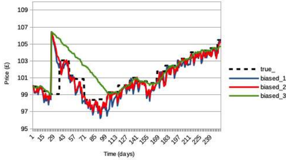
Fig. 2 Examples of fundamental values modelled by \mathcal{T}^j(t) (black dashed curve) and some agent’s approximation thereof as B^{i,j}(t) (continuous blue, red, and green curves) over a simulated time of one year.
