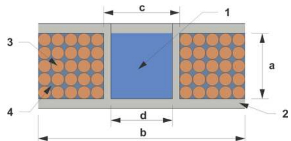
Fig. 1. The schematic of the vertical slice of the 25 windings ( 5 \times 5 ) coil that is used in the model, where 1: cell medium; 2: plastic coating of the cuvette; 3: insulated copper wire; 4: epoxy insulation.
