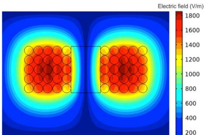
Fig. 3. Distribution of the induced electric field during highest dB/dt of the 5 \times 5 coil.
