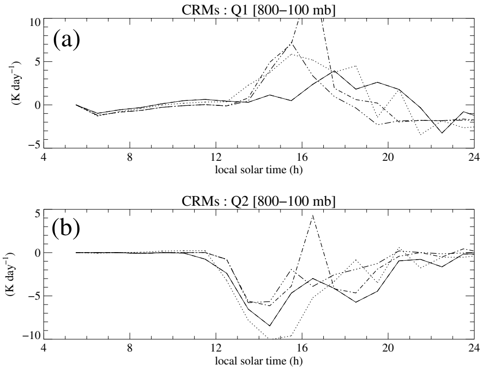
Figure 11. Time-series of the one-hour means forecast by the CRMs of (a) Q_1 and (b) Q_2 averaged over the layer 800–100 hPa.
