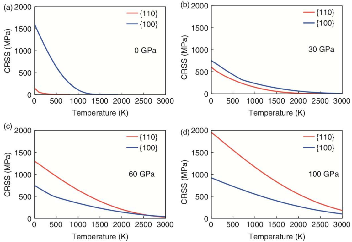
Figure 6. Critical resolved shear stress versus temperature for both \frac{1}{2}\langle 110 \rangle\{110\} (red curve) and \frac{1}{2}\langle 110 \rangle\{100\} (blue curve) as a function of pressure: (a) ambient pressure; (b) 30 GPa; (c) 60 GPa; (d) 100 GPa.
