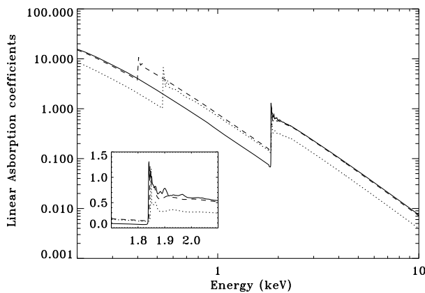
Fig. 4. Linear absorption coefficients of the CCD-22 compounds: (solid line) Si; (dotted line) \text{SiO}_2 ; (dashed line) \text{Si}_3\text{N}_4 . The small inset shows the XAFS just above the Si edge. The energy of the Si edge is slightly different depending on the compound considered. This is due to differences in the crystal lattice structure.
