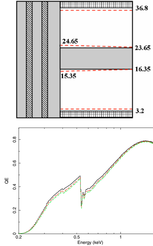
Fig. 21. (Top panel) Drawing showing the changes in the geometry of the finger and channel stop, corresponding to a reduction of the open area by 10.6%. (Bottom panel) Plot of the low-energy quantum efficiency for different configurations of the geometry of the CCD pixel: (black) using the default CCD geometry shown in Fig. 3; (red) with an increase of the width of each channel stop by 1 \mu\text{m} ; (green) with an increase of the width of each channel stop by 1 \mu\text{m} and the finger structure as shown in the top panel.
