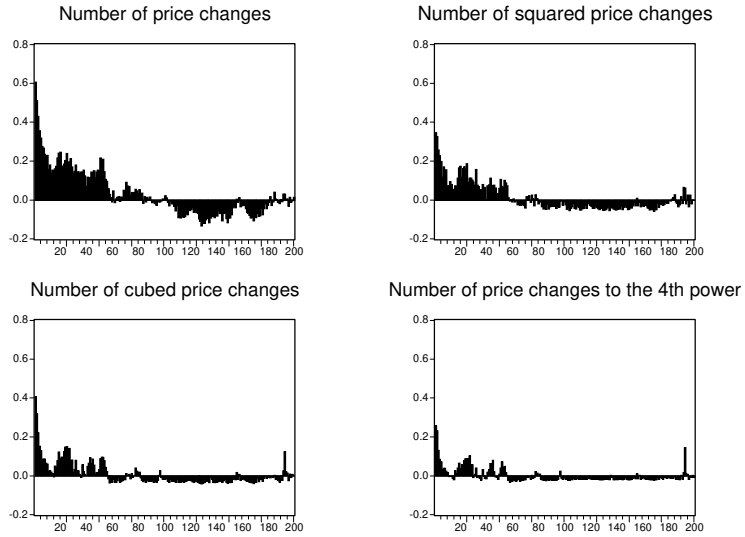
Figure 8: Autocorrelations of the daily number of price changes larger than $ .75 on IBM
