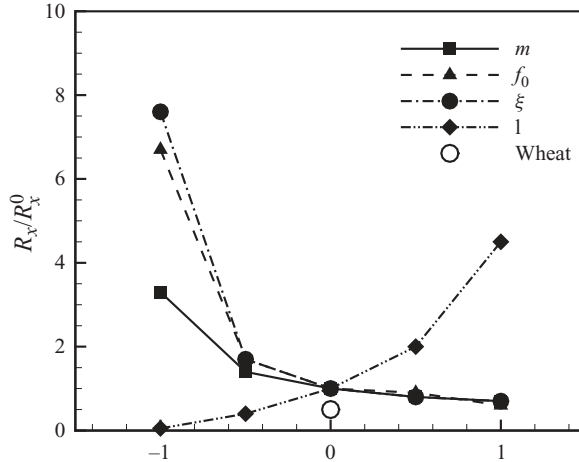
FIGURE 16. Sensitivity to the plant mechanical properties of the normalized streamwise r.m.s. difference between the drag terms at canopy top for waving and fixed plants. On the horizontal axis the coded values of plant mechanical properties refer to the values indicated in table 3. Each plain dot represents one run where only one parameter (mass m , natural vibration frequency f_0 , damping coefficient \xi and plant spacing l ) was modified compared to others that were kept at their reference value (coded value equal to 0).
