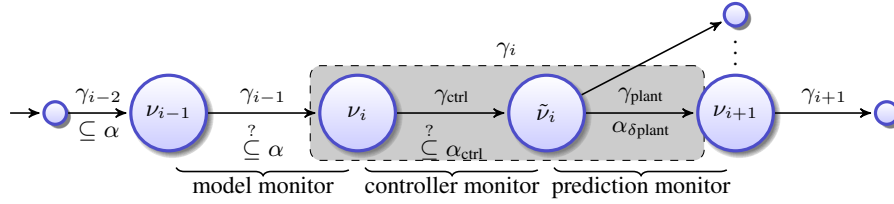
Fig. 1: Use of ModelPlex monitors along a system execution
