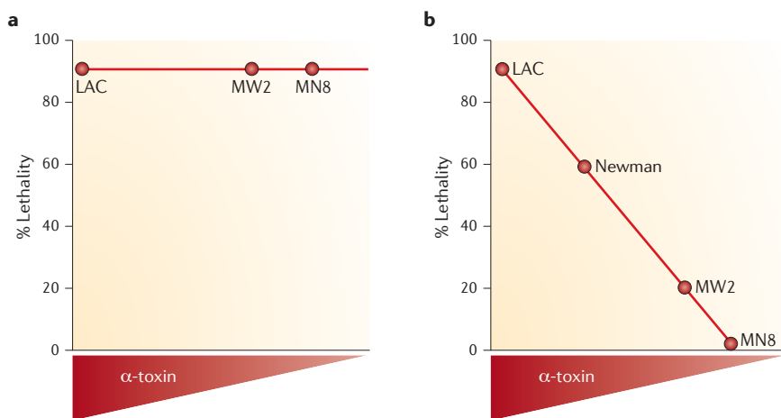
Figure 2 | Lethality induced by various Staphylococcus aureus strains as a function of the animal model used (mouse versus rabbit pneumonia model) and their level of α-toxin production. a | Inoculation of the S. aureus strains LAC, MW2 and MN8 at 6.5 × 10 8 CFUs per kg in the rabbit pneumonia model shows that they are equally virulent 48 hours after infection. b | Inoculation of the S. aureus strains LAC, Newman, MW2 and MN8 at 6.5–10 × 10 9 CFUs per kg in the mouse pneumonia model shows that virulence correlates with the level of α-toxin production. Data taken from REFS 46,48,50,51.
