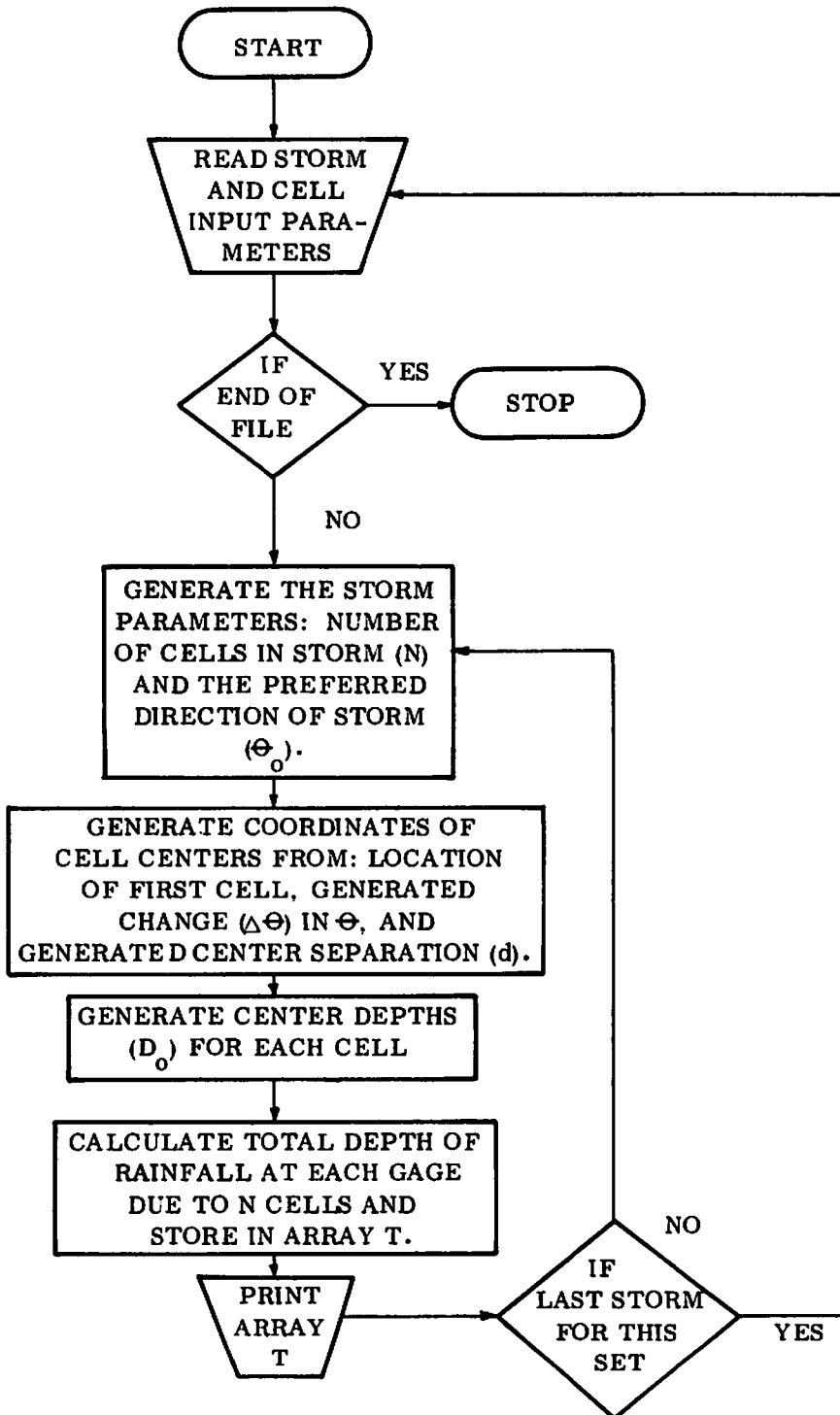
FIGURE 5—Flow chart for simulation of individual airmass thunderstorm rainfall.
