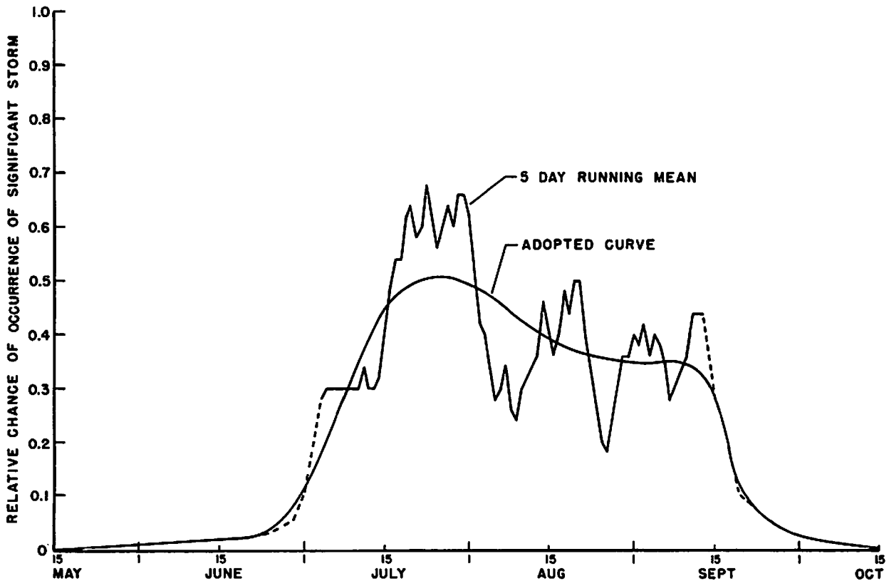
FIGURE 3.—Empirically derived curve for the probability of significant storms on Walnut Gulch watershed.
