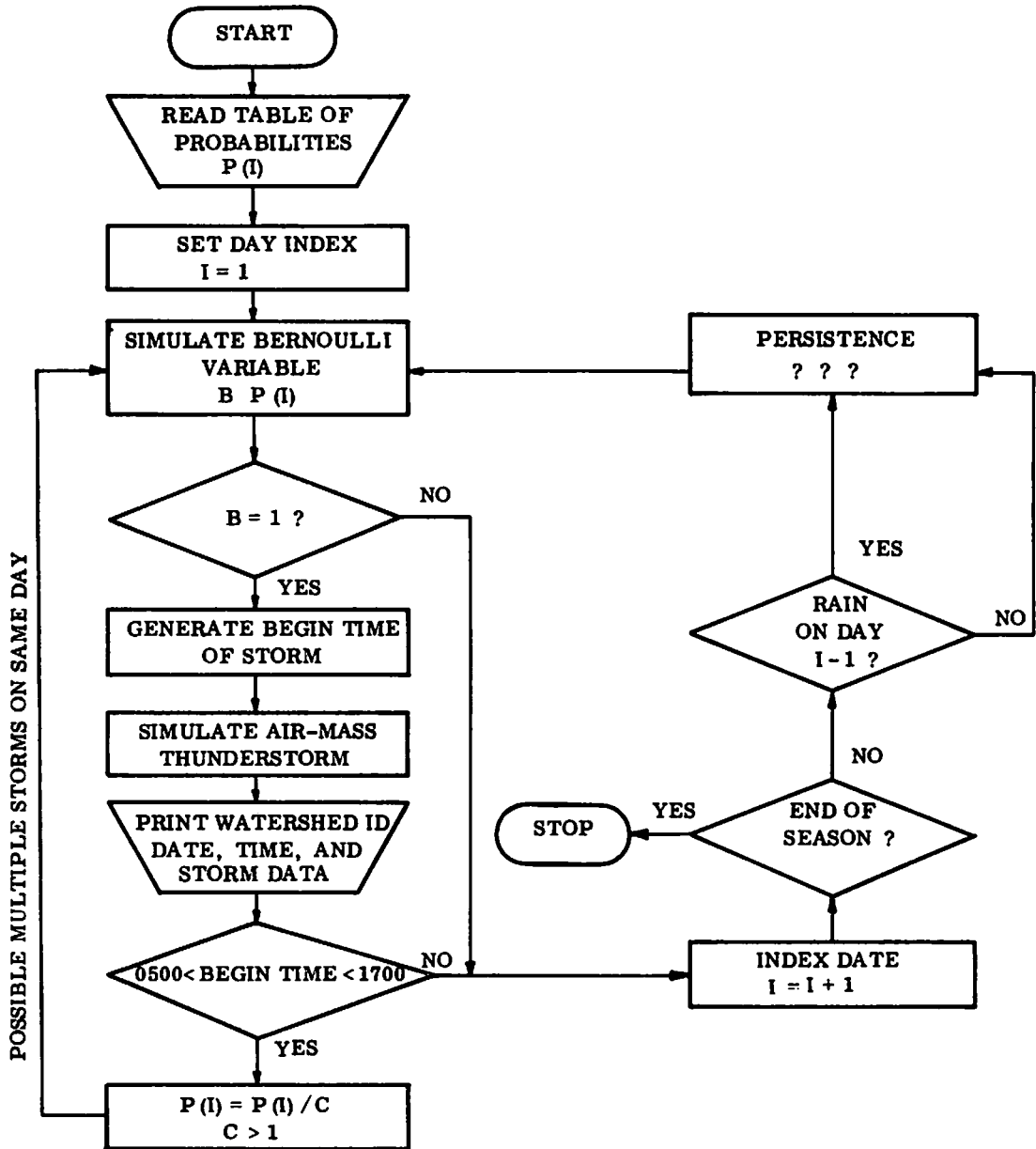
FIGURE 4. — Flow chart for generation of seasonal synthetic rainfall data.
