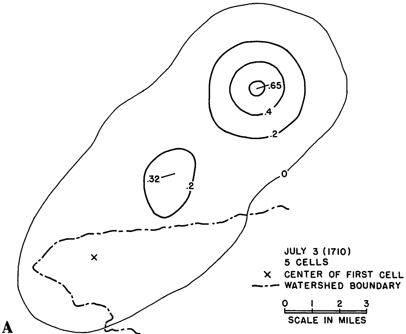
FIGURE 7.—Isohyetal maps of selected synthetic thunderstorm events: A. July 3 (1710) 5 cells center of first cell watershed boundary. B. July 4 (1723) 3 cells center of first cell watershed boundary. C. July 9 (1733) 4 cells center of first cell watershed boundary. D. Aug. 15 (1300) 5 cells center of first cell watershed boundary. E. Aug. 16 (1957) 5 cells center of first cell watershed boundary. F. Aug. 29 (1641) 5 cells center of first cell watershed boundary. G. Sept. 11 (1641) 5 cells center of first cell watershed boundary. H. Sept 13 (1835) 5 cells center of first cell watershed boundary.
