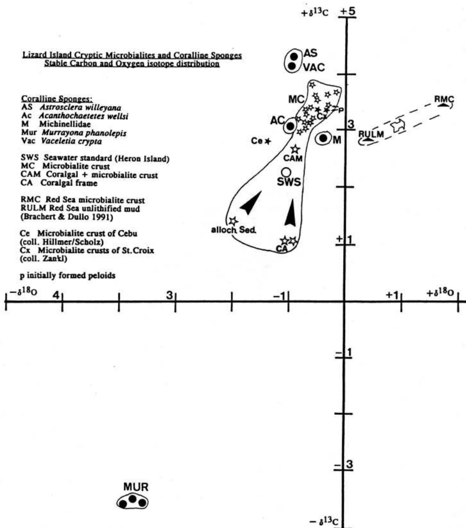
Fig. 7. Distribution pattern \delta^{13}\text{C} and \delta^{18}\text{O} (v. PDB) of modern cryptic microbialites from Lizard Island, St. Croix and Cebu (Philippines), and coralline sponges.
