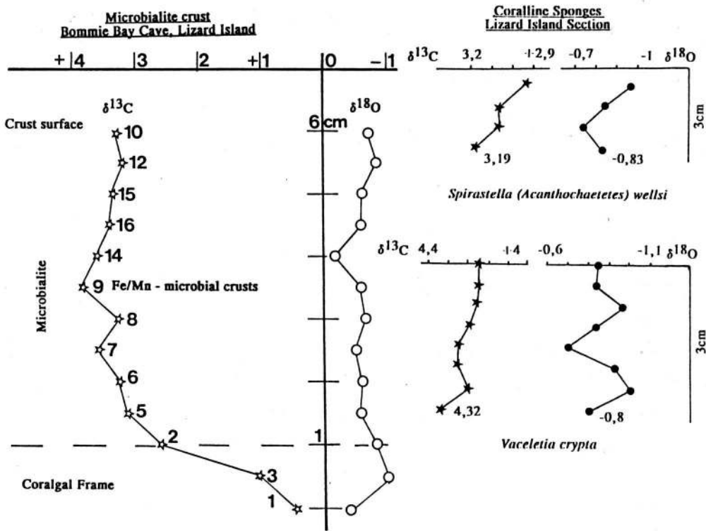
Fig. 8. Stable carbon and oxygen isotope profile from a Bommie Bay research cave microbialite (versus PDB standard).
