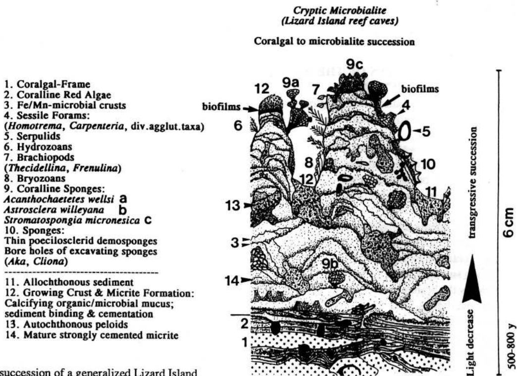
Fig. 4. Facies succession of a generalized Lizard Island type microbialite.
