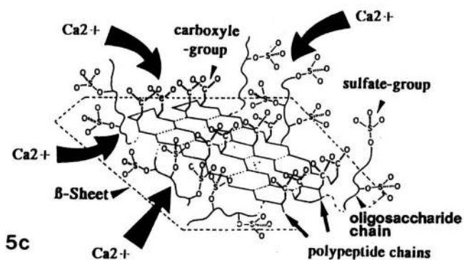
Fig. 5. Mineralization model via Ca-binding organic macromolecules.
