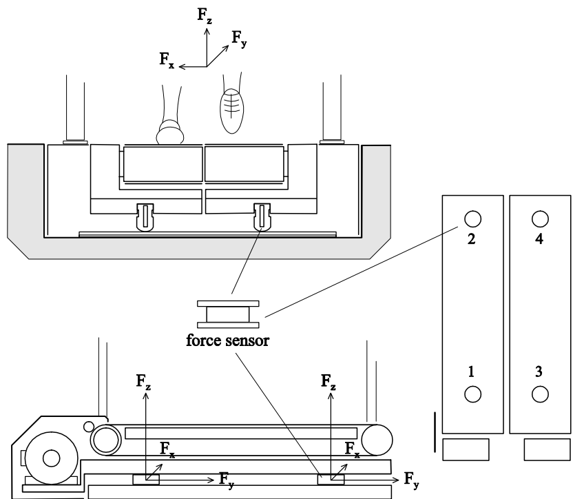
Fig. 9. ADAL3D-F concept.
