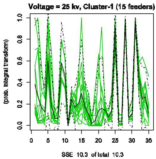
Figure 5: Cluster analysis for region 2, 25 kV, one cluster
