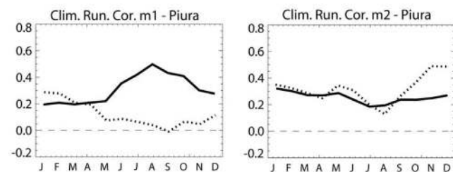
Figure 8. Climatology of the 60 day (120 day) running correlation between the SVD time series for SST and wind stress for modes (a) one and (b) two. The solid (dotted) line is for the 1–30 day ([30, \infty ] day) period band. Correlation above 0.2 are significant at the level \sigma = 95\% .
