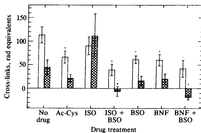
FIG. 2. DNA cross-links in chicken embryo hepatocytes produced by chromium(VI) after various drug treatments. Cells were treated as described in Fig. 1 legend. Open bars, total DNA cross-links (without proteinase K digestion); cross-hatched bars, DNA interstrand cross-links (with proteinase K digestion of the cell lysates). Values represent mean \pm SEM for n \geq 6 .
