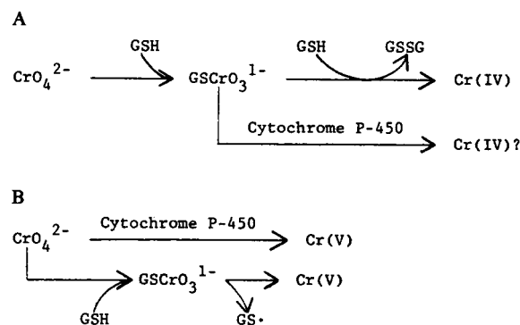
FIG. 3. Possible metabolic pathways of chromium(VI) in cells. (A) Under conditions with high GSH levels. (B) Under conditions with low GSH levels. GSSG, glutathione disulfide; \text{GS}\cdot , glutathione radical. See ref. 12 for the GSSG pathway in A and refs. 33 and 32, respectively, for the cytochrome P-450 and GSH pathways in B.
