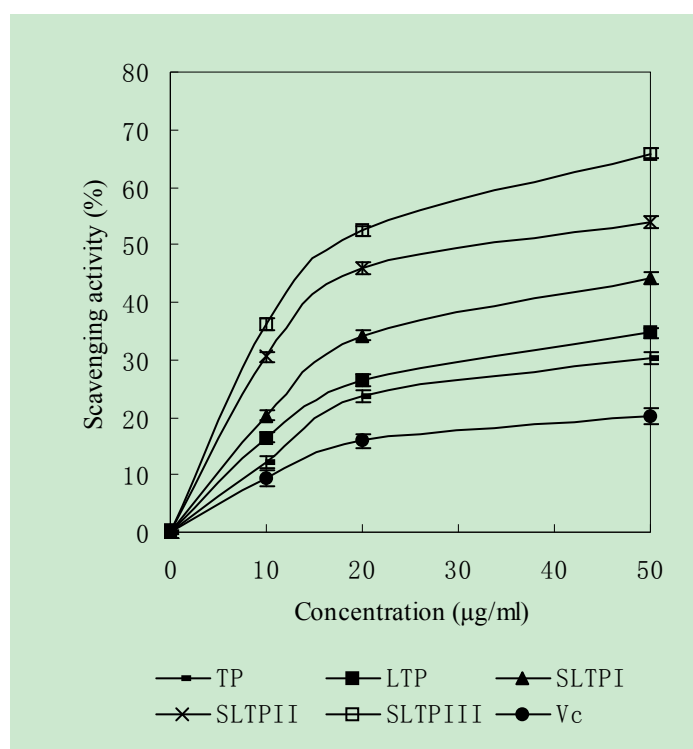
Figure 3. Scavenging activity of natural TP, its derivatives and Vitamin C against hydroxyl radicals. Values were means ± SD (n = 3).
