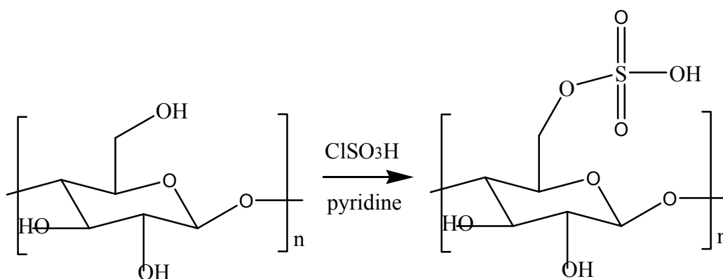
Figure 1. Sulfation of LTP.
