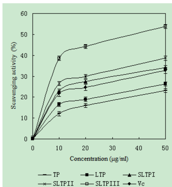
Figure 2. Scavenging activity of natural TP, its derivatives and Vitamin C against DPPH radicals. Values were means \pm SD (n = 3).
