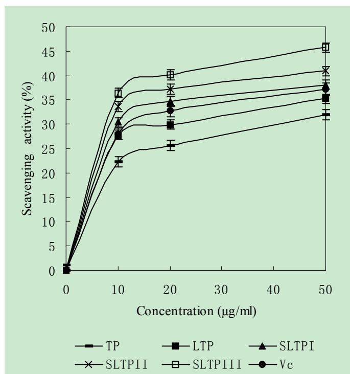
Figure 4. Scavenging activity of natural TP, its derivatives and Vitamin C against superoxide anion radicals. Values were means ± SD (n = 3).
