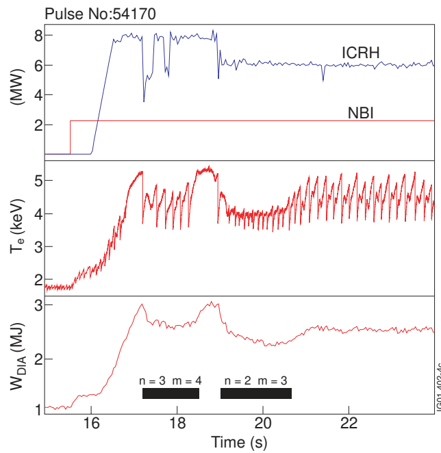
FIGURE 2 ICRF and NBI power, electron temperature and diamagnetic plasma energy for discharge 54170 with \omega \approx 3\omega(^4\text{He}) and 120 keV deuterium NBI. Also shown are the time intervals where NTMs with n=3/m=4 and n=2/m=3 , triggered by the crashes of long-period sawteeth, are observed.
