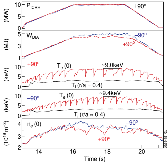
FIGURE 3 ICRF power, diamagnetic plasma energy, central electron temperature, ion temperature at r/a = 0.4 and central electron density for two discharges with different ICRF phasings (discharges 41514 and 41515).
