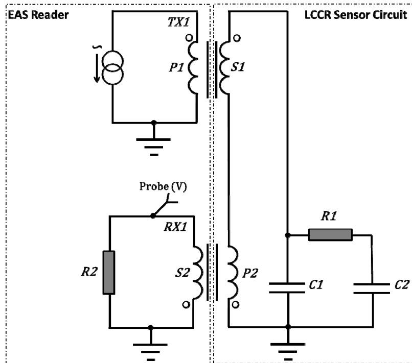
Figure 2. Electrical layout used for the simulation of the Electronic Article Surveillance (EAS) tag reader and EAS tag.
