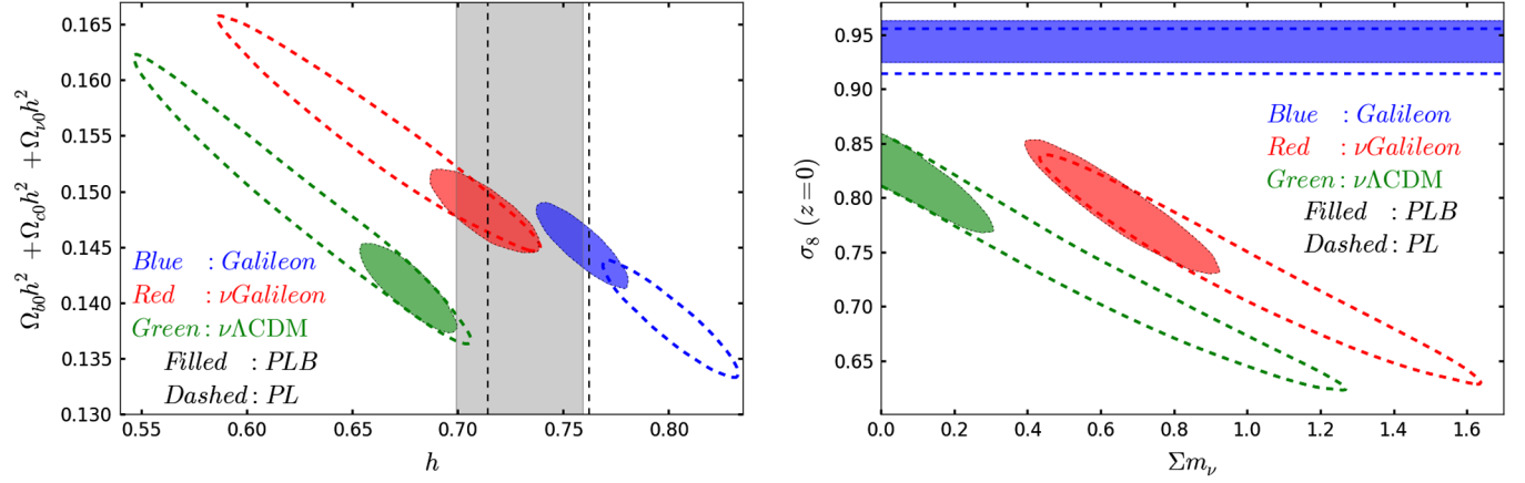
FIG. 1 (color online). Marginalized two-dimensional 95% confidence limit contours obtained using the PL (open dashed) and PLB (filled) data sets for the base Galileon (blue), \nu Galileon (red) and \nu\Lambda CDM (green) models. In the left panel, the vertical bands indicate the 68% confidence limits of the direct measurements of h presented in Ref. [30] (open dashed) and Ref. [31] (grey filled). In the right panel, the horizontal bands indicate the 95% confidence interval on \sigma_8 obtained using the PL (open dashed) and PLB (blue filled) data sets for the base Galileon model (which does not contain massive neutrinos).
