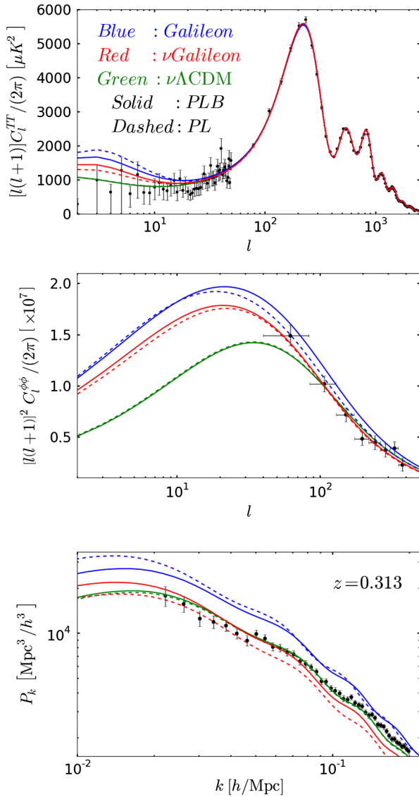
FIG. 2 (color online). CMB temperature anisotropy (top), CMB lensing (middle) and linear matter power spectra (bottom) of the best-fitting base Galileon (blue), \nu\text{Galileon} (red) and \nu\Lambda\text{CDM} (green) models for the PL (dashed) and PLB (solid) data sets. In the upper and middle panels, the data points show the power spectrum measured by the Planck satellite [25,26]. In the lower panel, the data points show the SDSS-DR7 Luminous Red Galaxy host halo power spectrum as presented in Ref. [32], but scaled down to match approximately the amplitude of the best-fitting \nu\text{Galileon} ( PLB ) model.
