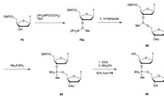
Scheme 32 Synthesis of BMP-dithymidine 90 .
