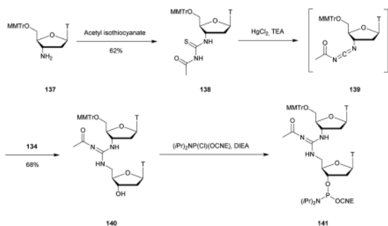
Scheme 43 Synthesis of acetylguanidine-dithymidine phosphoramidite building block 141 .
