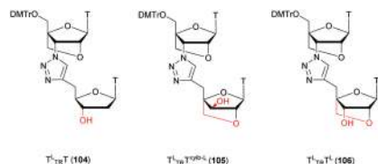
Fig. 18 Chemical structures of T^L\text{-TrT} ( 104 ), T^L\text{-TrT}^{\text{xylo-L}} ( 105 ) and T^L\text{-TrT}^L ( 106 ) TR-LNA-dithymidines.
