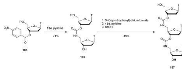
Scheme 54 Synthesis of 5'- N -CA trinucleoside 187 .
