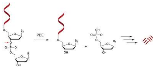
Scheme 1 General representation of the hydrolysis of an ODN by a 5'-PDE.
