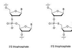
Scheme 9 Chemical structures of 3'-S and 5'-S thiophosphate linkages.
