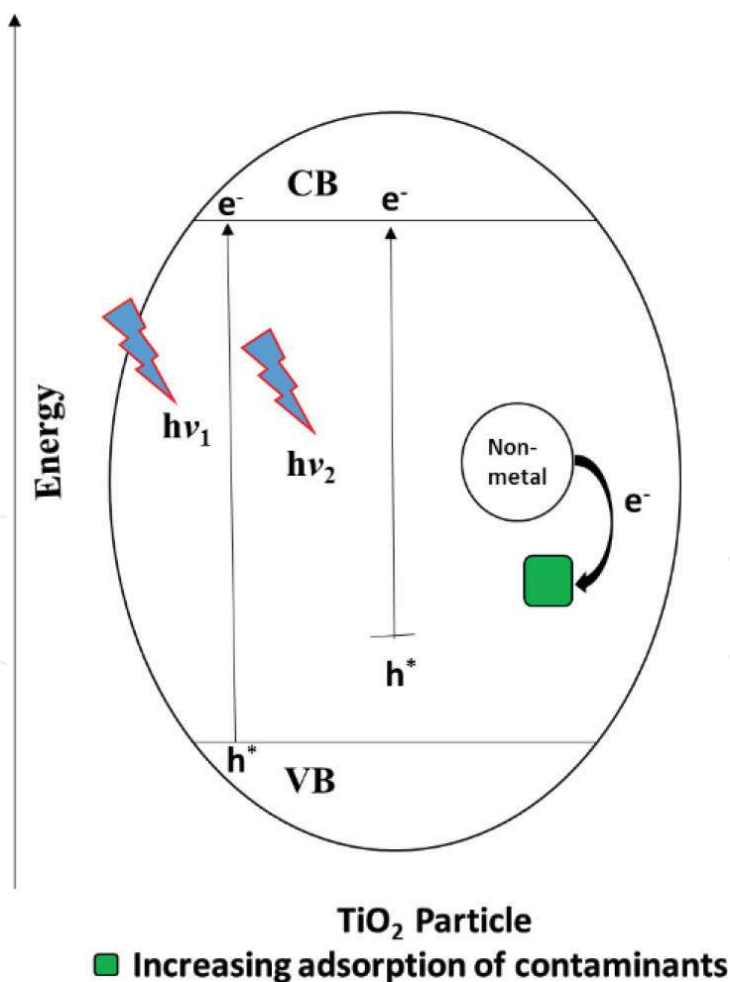
Figure 2. Band-gap energy narrowing mechanism for non-metal-doped TiO 2 .
