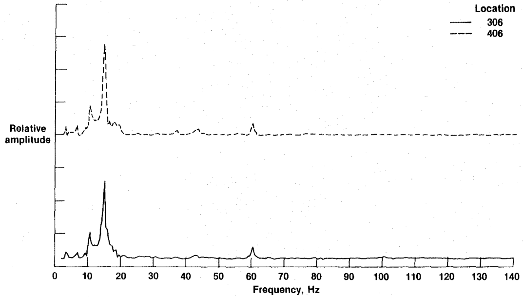
Figure 35. Location 306 and 406 vertical frequency responses due to antisymmetric sweep at each engine (full fuel tanks).
