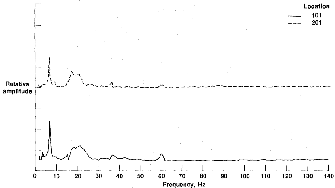
Figure 30. Location 101 and 201 vertical frequency responses due to symmetric sweep at each engine (full fuel tanks).
