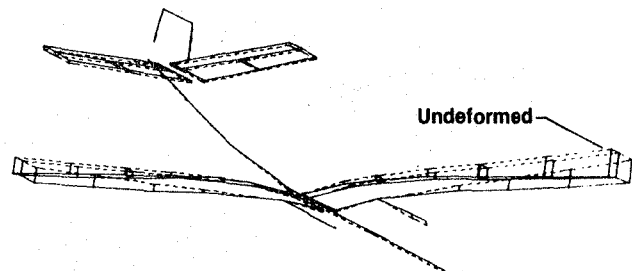
Figure 12. Symmetric wing bending mode shape (full fuel tanks), 6.86-Hz frequency.
