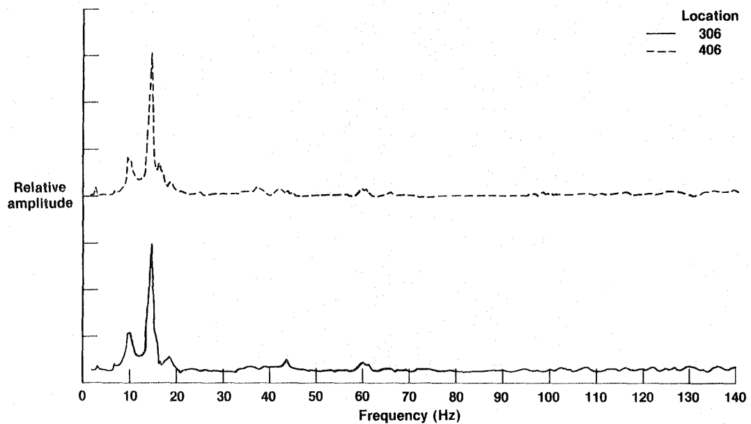
Figure 48. Location 306 and 406 vertical frequency responses due to antisymmetric sweep at each wingtip (full fuel tanks).
