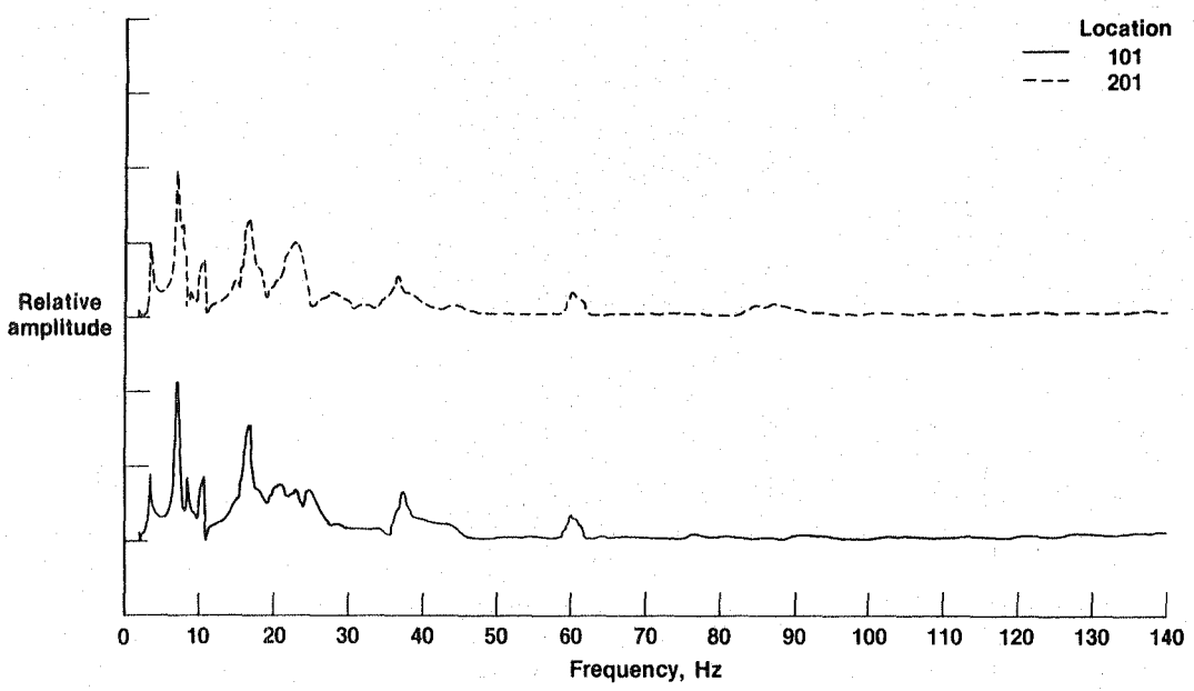
Figure 56. Location 101 and 102 vertical frequency responses due to antisymmetric sweep at each engine (empty fuel tanks).
