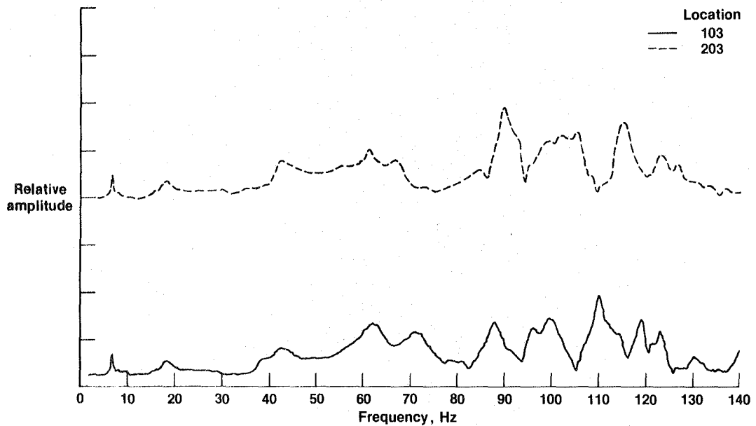
Figure 44. Location 103 and 203 vertical frequency responses (10-lb preload) due to symmetric sweep at each wingtip (full fuel tanks).
