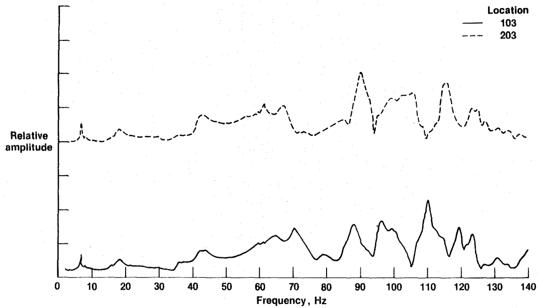
Figure 43. Location 103 and 203 vertical frequency responses due to symmetric sweep at each wingtip (full fuel tanks).
