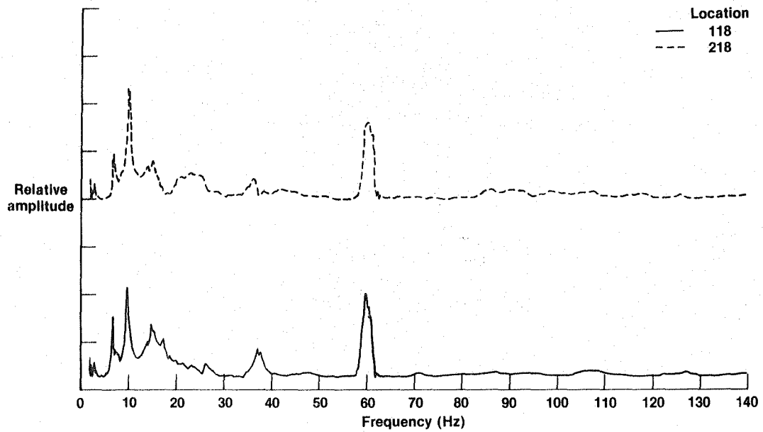
Figure 47. Location 118 and 218 lateral frequency responses due to antisymmetric sweep at each wingtip (full fuel tanks).
