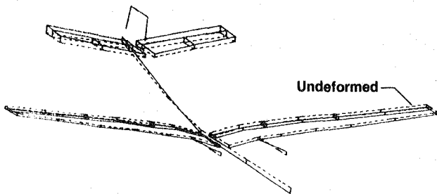
Figure 24. Symmetric engine pitch mode shape (empty fuel tanks), 9.47-Hz frequency.
