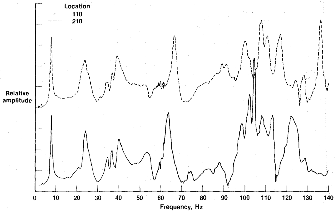
Figure 65. Location 110 and 210 vertical frequency responses (10-lb preload) due to symmetric sweep at each wingtip (empty fuel tanks).
