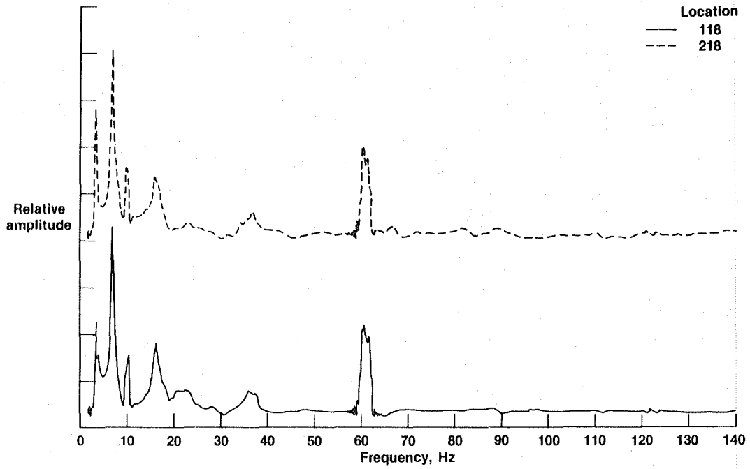
Figure 69. Location 118 and 218 vertical frequency responses due to antisymmetric sweep at each wingtip (empty fuel tanks).
