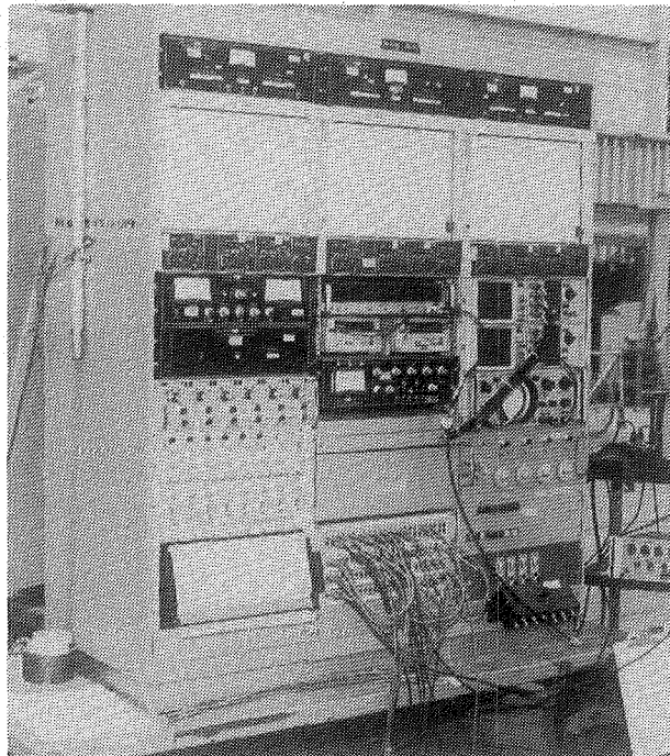
Figure 3. Sine dwell ground vibration test equipment.
