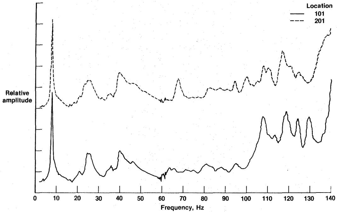
Figure 59. Location 101 and 201 vertical frequency responses due to symmetric sweep at each wingtip (empty fuel tanks).
