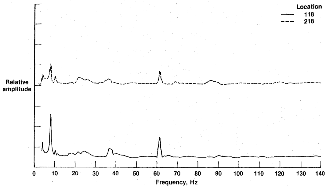
Figure 60. Location 118 and 218 vertical frequency responses due to symmetric sweep at each wingtip (empty fuel tanks).
