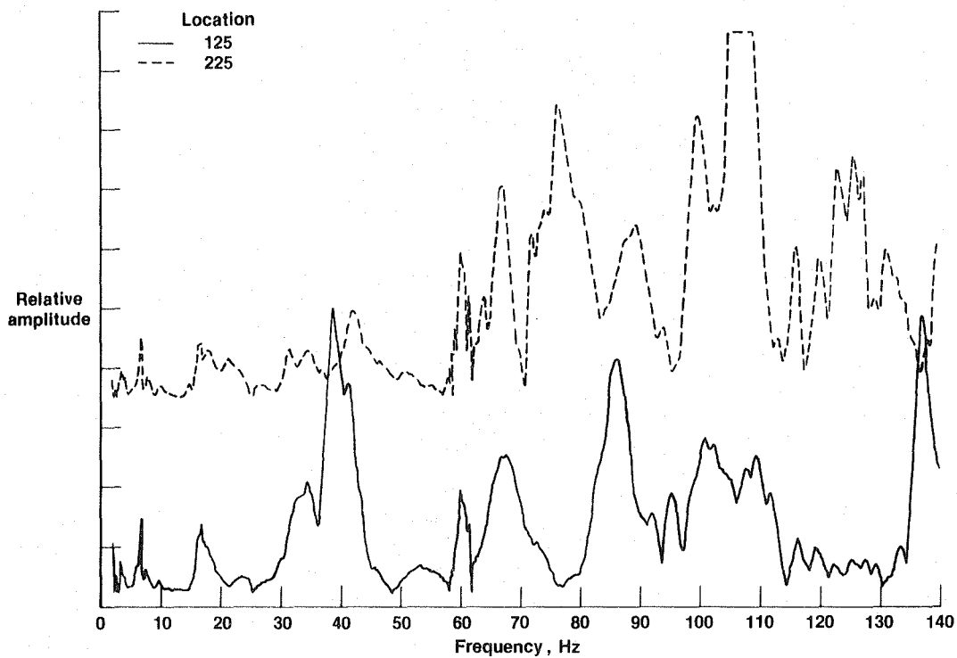
Figure 42. Location 125 and 225 vertical frequency responses due to symmetric sweep at each wingtip (full fuel tanks).
