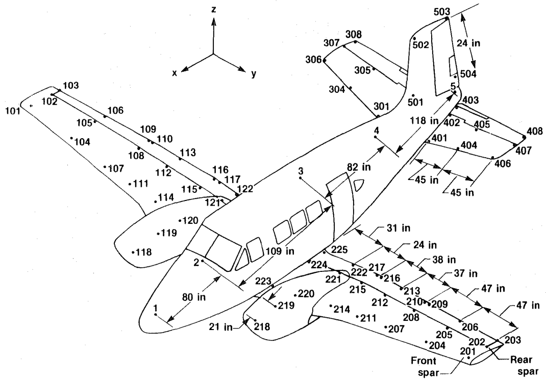
Figure 6. U-8F accelerometer locations for mode shape measurements.
