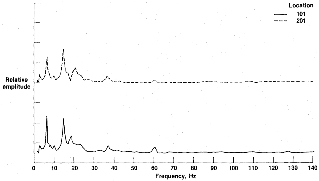
Figure 33. Location 101 and 201 vertical frequency responses due to antisymmetric sweep at each engine (full fuel tanks).
