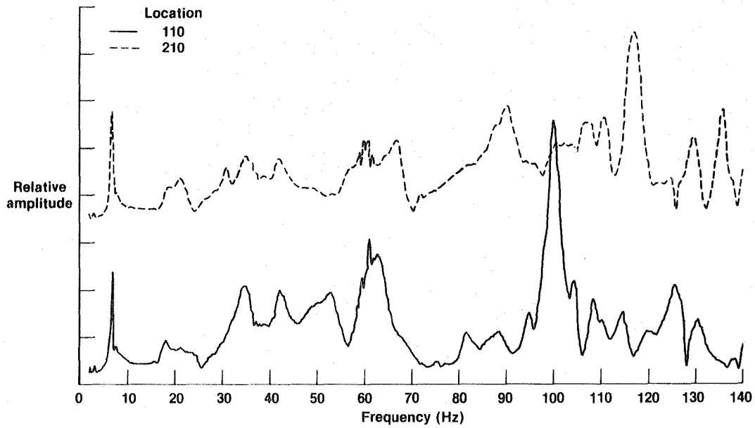
Figure 41. Location 110 and 210 vertical frequency responses (10-lb preload) due to symmetric sweep at each wingtip (full fuel tanks).
