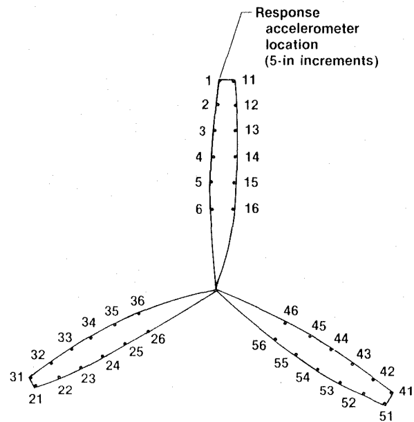
Figure 7. U-8F propeller impact hammer excitation locations.
