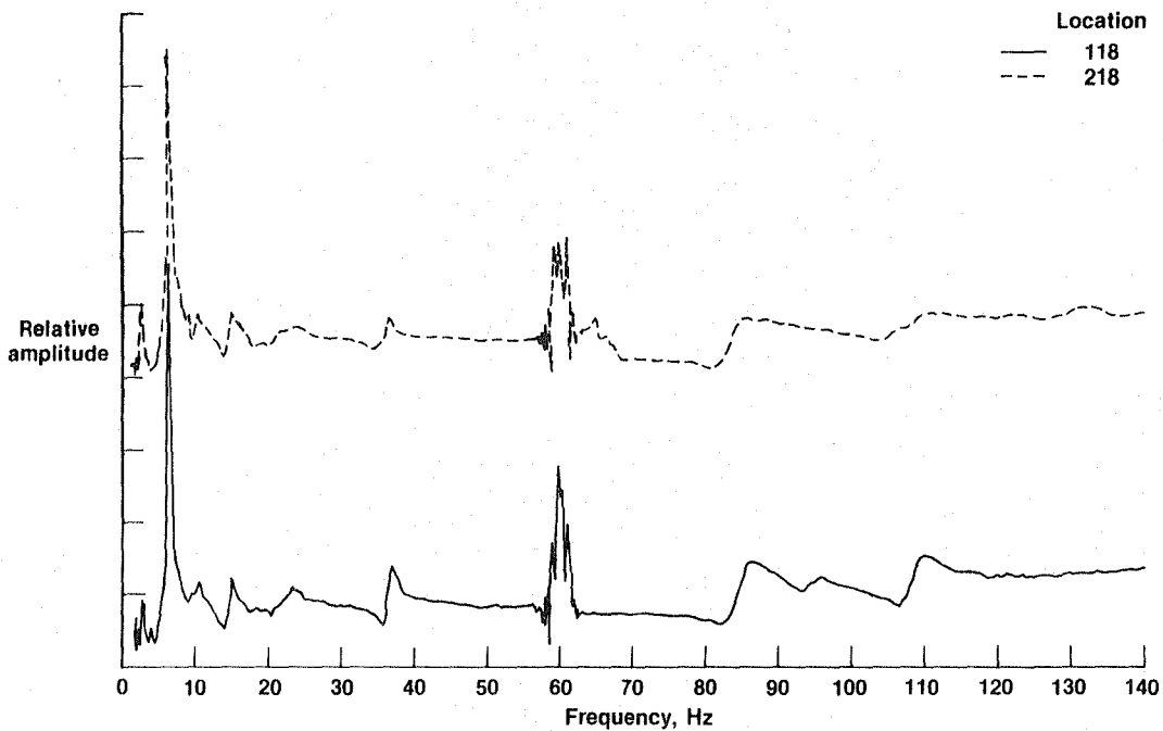
Figure 34. Location 118 and 218 vertical frequency responses due to antisymmetric sweep at each engine (full fuel tanks).
