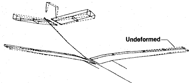
Figure 25. Fuselage torsion mode shape (empty fuel tanks), 10.56-Hz frequency.
