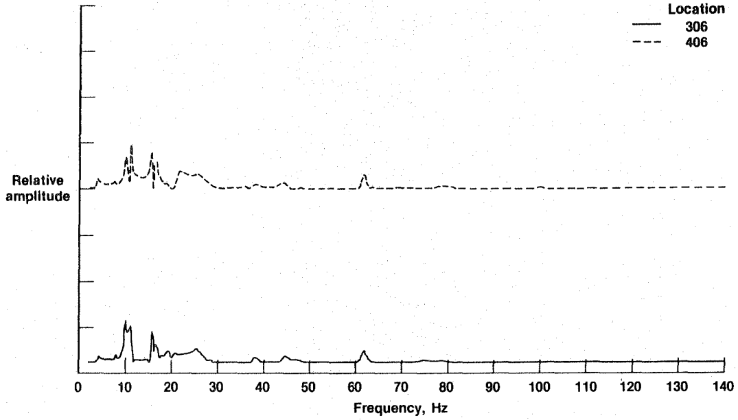
Figure 55. Location 306 and 406 vertical frequency responses due to symmetric sweep at each engine (empty fuel tanks).
