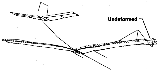
Figure 19. Aileron bending mode shape (full fuel tanks), 41.18-Hz frequency.
