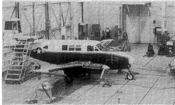
Figure 2. Ground vibration test setup.
