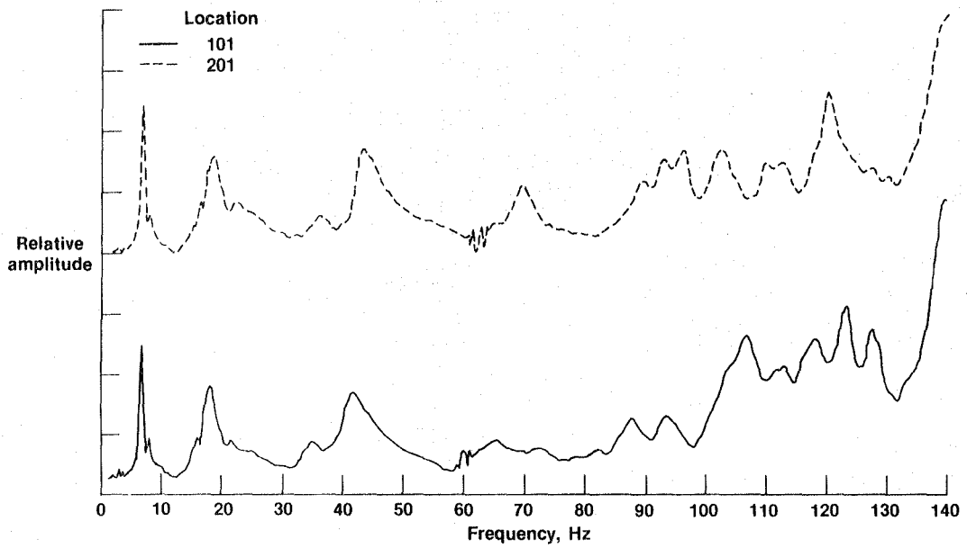
Figure 36. Location 101 and 201 vertical frequency responses due to symmetric sweep at each wingtip (full fuel tanks).
