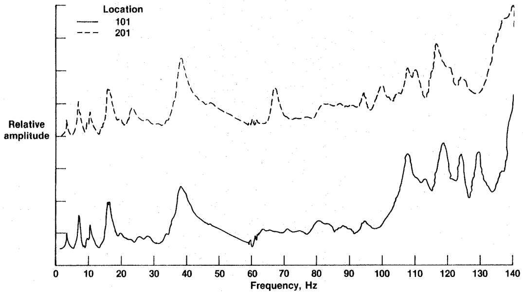
Figure 68. Location 101 and 201 vertical frequency responses due to antisymmetric sweep at each wingtip (empty fuel tanks).
