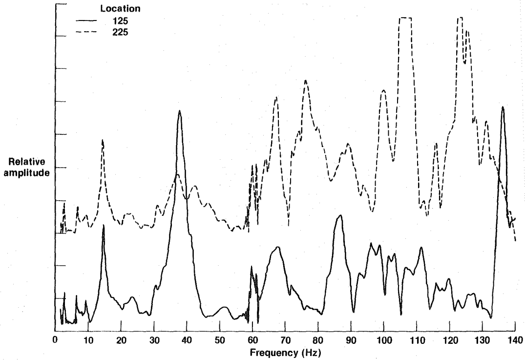
Figure 49. Location 125 and 225 vertical frequency responses due to antisymmetric sweep at each wingtip (full fuel tanks).
