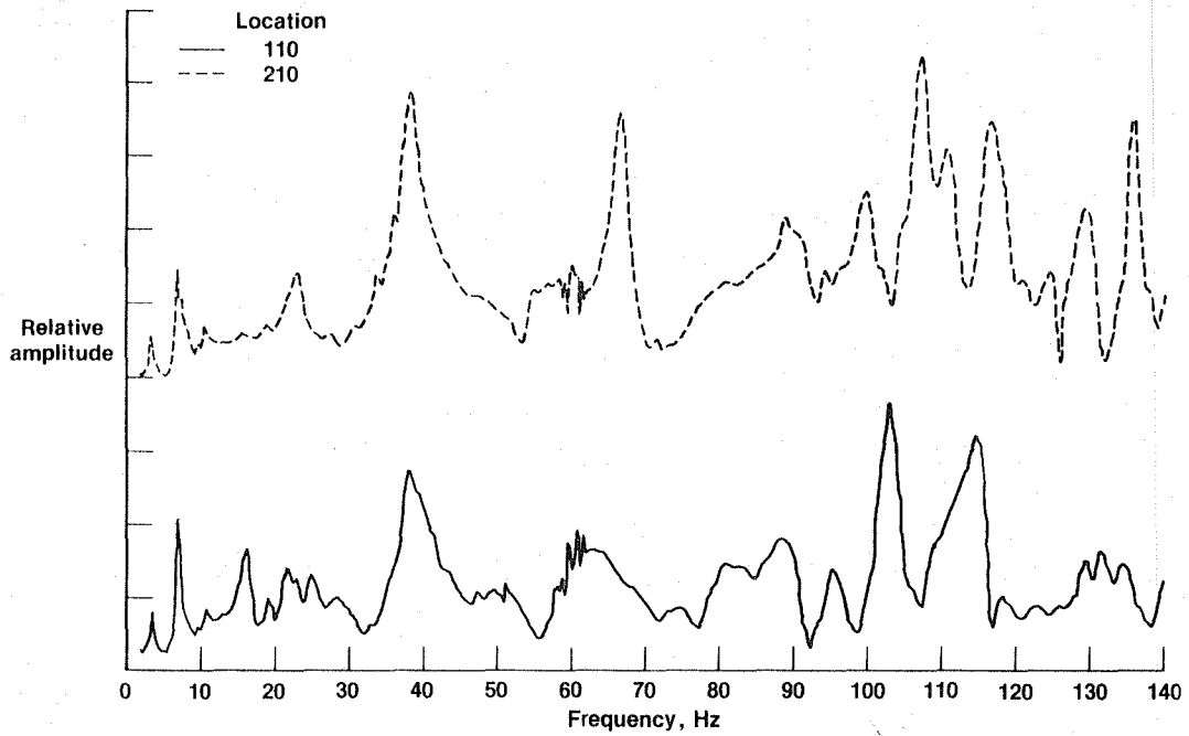
Figure 74. Location 110 and 210 vertical frequency responses due to antisymmetric sweep at each wingtip (empty fuel tanks).
