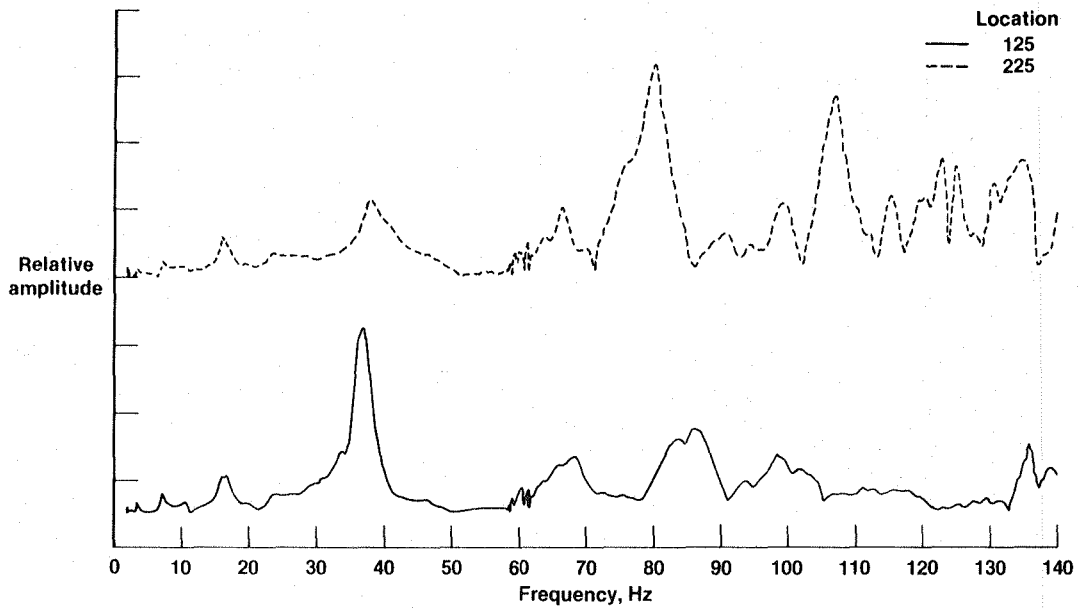
Figure 73. Location 125 and 225 lateral frequency responses due to antisymmetric sweep at each wingtip (empty fuel tanks).
